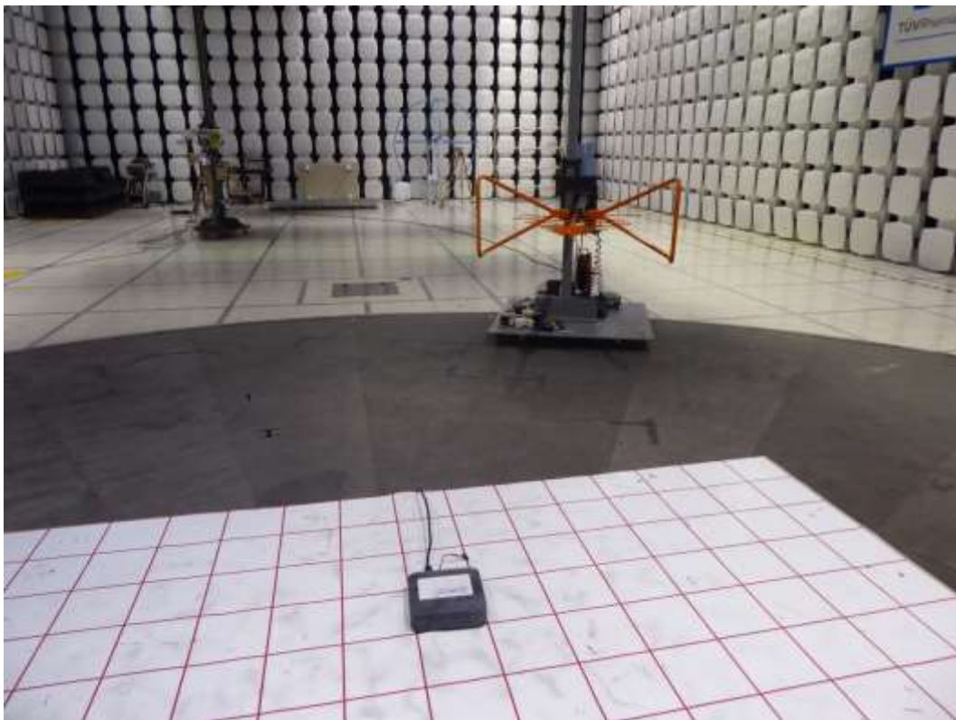
Figure 3 – 30 – 1000 MHz 3 meter Radiated Setup
