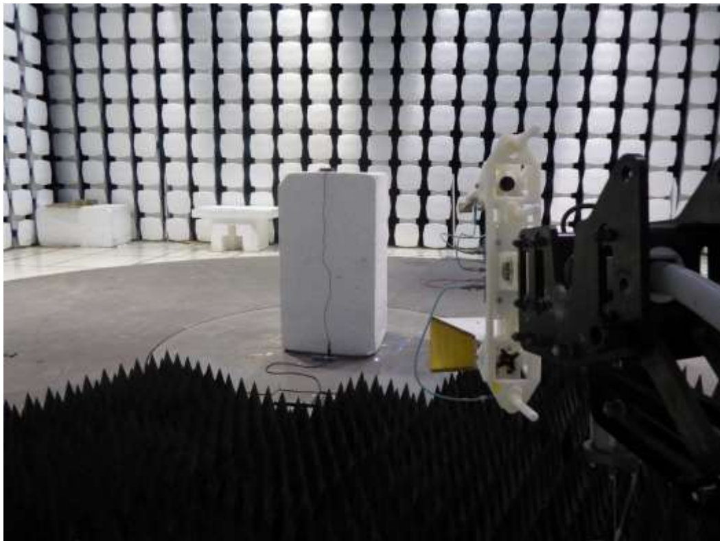
Figure 6 – 1 – 18 GHz 3 meter Radiated Test Setup
