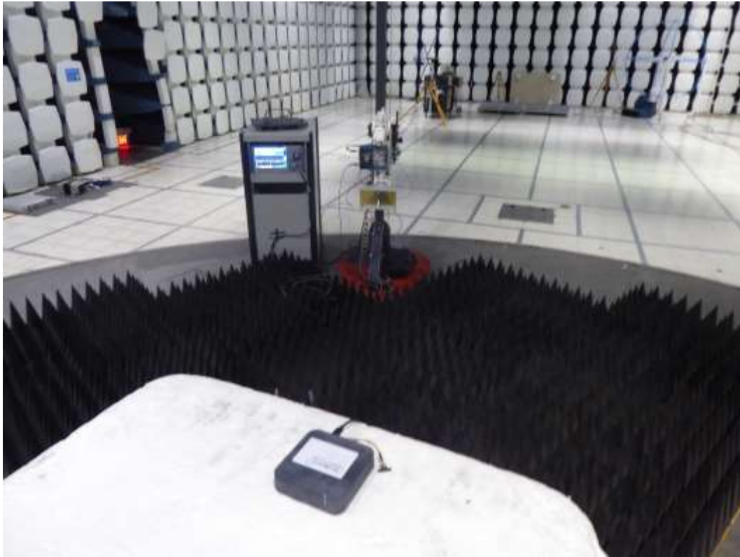
Figure 5 – 1 – 18 GHz 3 meter Radiated Setup
