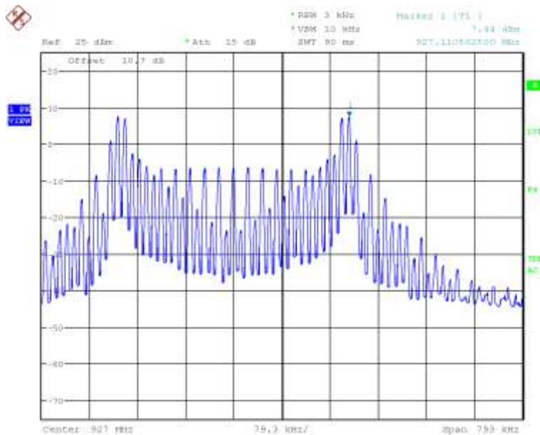
Figure 23 – Mid Channel Power Spectral Density (FSK)
