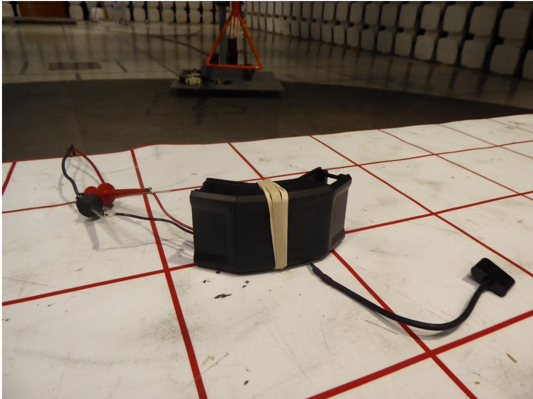
Figure 1 – External Photo of EUT
