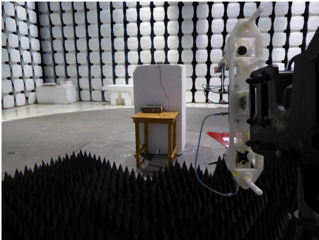
Figure 7 – 1 – 18 GHz 3 meter Radiated Test Setup
