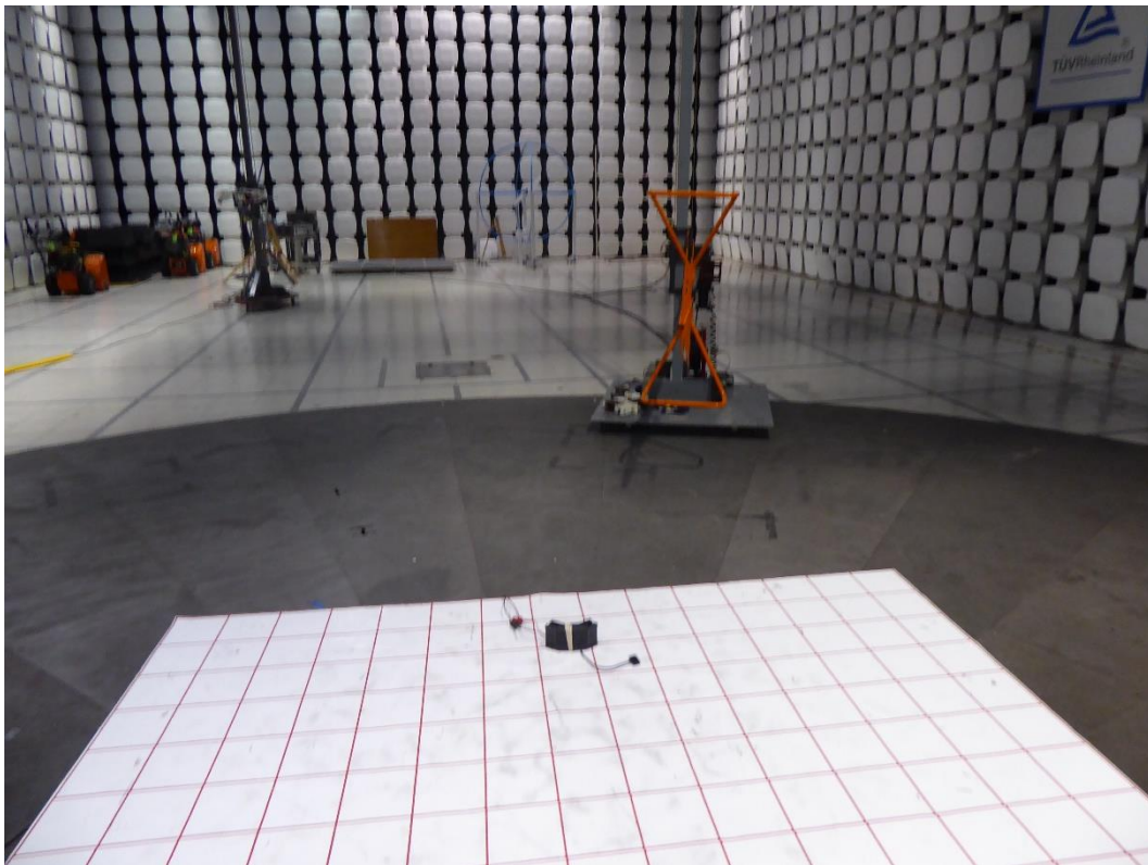
Figure 4 – 30 – 1000 MHz 3 meter Radiated Setup
