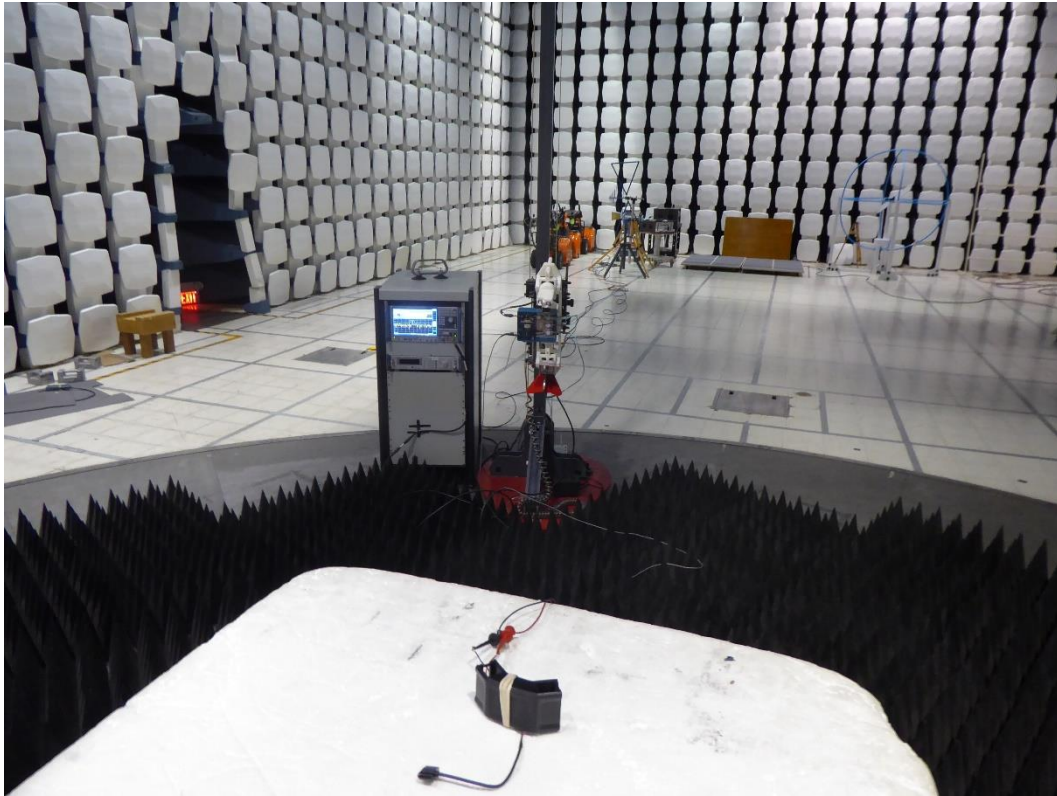
Figure 6 – 1 – 18 GHz 3 meter Radiated Setup
