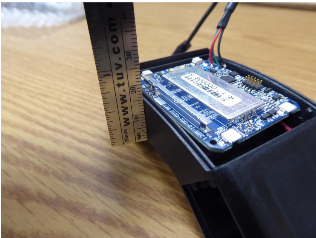
Figure 3 – Internal Photo of EUT (Antenna Distance to Limb)
