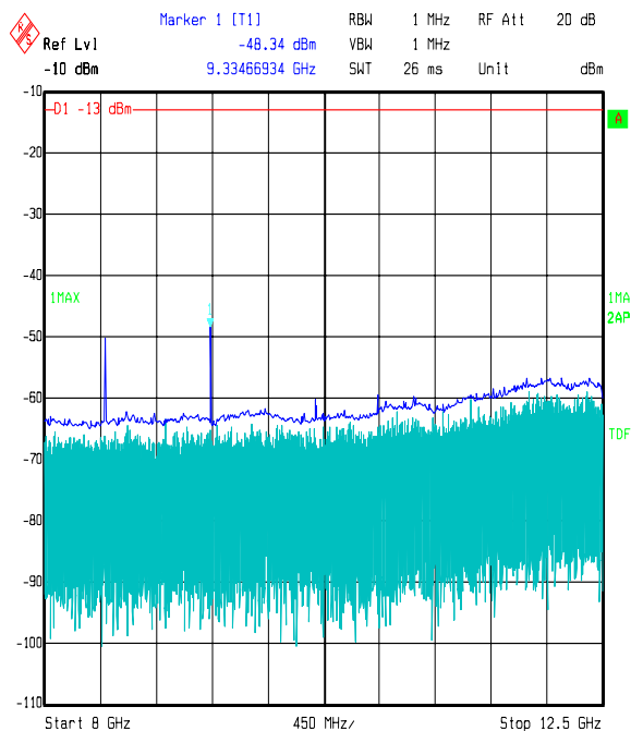
Title: Satellite Tracking People 48270 Comment A: FCC 22 Top channel Date: 14.MAY 2006 16:33:25
