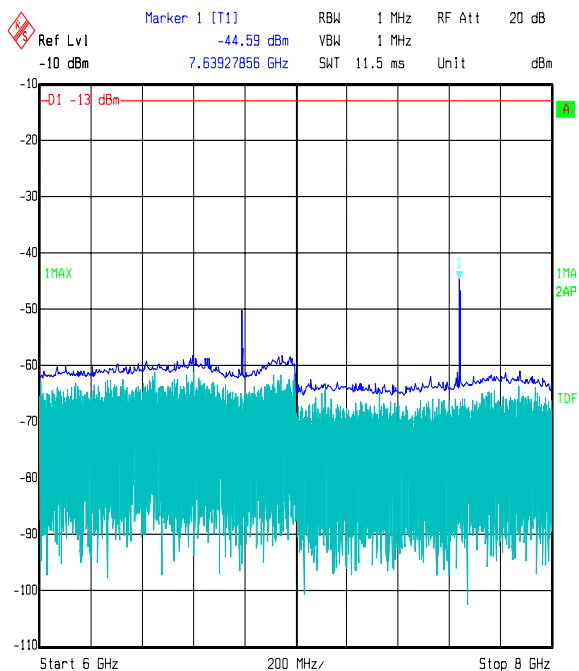
Title: Satellite Tracking People 48270 Comment A: FCC 22 Top channel Date: 14.MAY 2006 15:06:32
