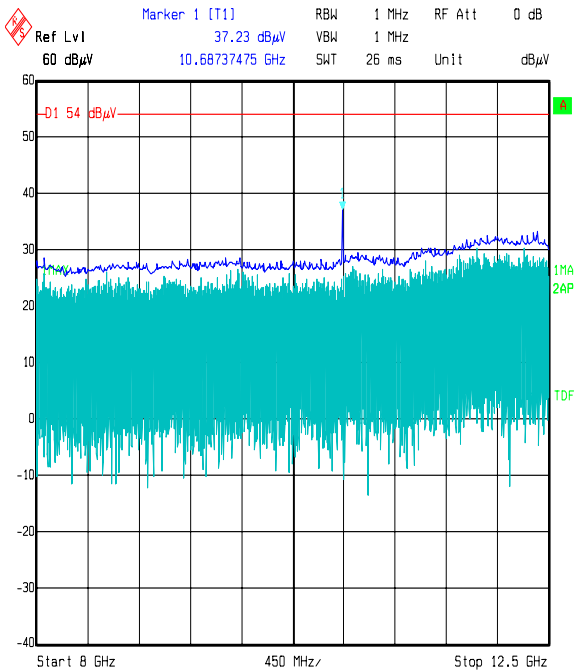
Title: Satellite Tracking People 48270 Comment A: FCC 22 Top,Mid, & Bot channel Date: 14.MAY 2006 18:36:16
