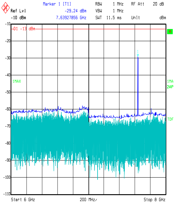
Title: Satellite Tracking People 48270 Comment A: FCC 24 Top channel Date: 14.MAY 2006 15:14:51
