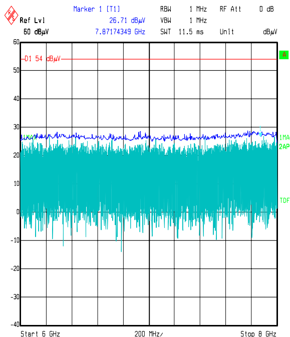
Title: Satellite Tracking People 48270 Comment A: FCC 24 Top,Mid, & Bot channel Date: 14.MAY 2006 18:13:21
