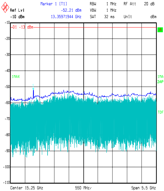
Title: Satellite Tracking People 48270 Comment A: FCC 24 Top channel Date: 14.MAY 2006 17:01:57
