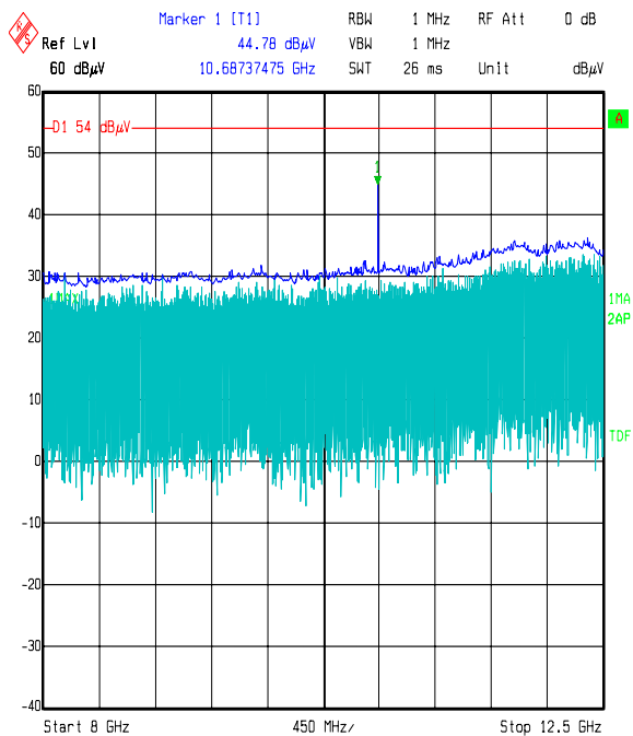
Title: Satellite Tracking People 4820 Comment A: FCC 24 Top,Mid, & Bot channel Date: 14.MAY 2006 18:41:42
