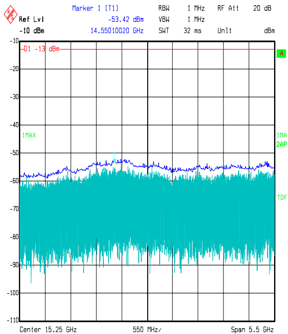
Title: Satellite Tracking People 48270 Comment A: FCC 22 Top channel Date: 14.MAY 2006 16:48:23
