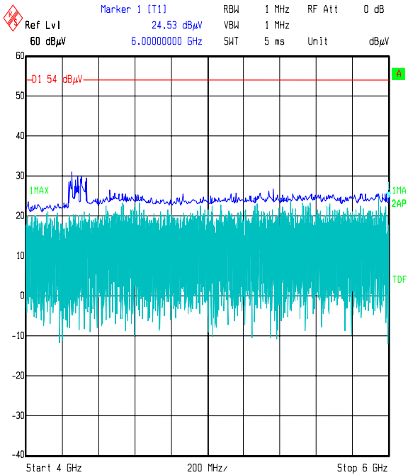
Title: Satellite Tracking People 48270 Comment A: FCC 22 Top,Mid, & Bot channel Date: 14.MAY 2006 17:51:14
