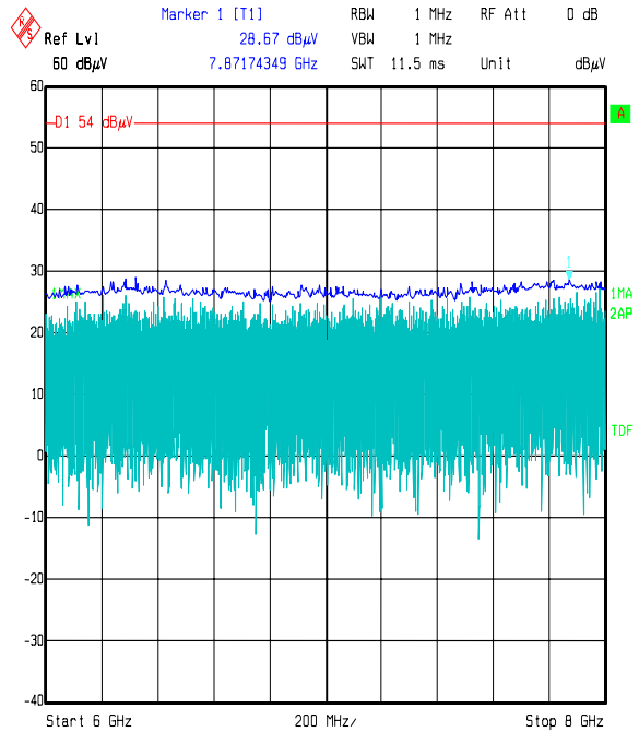
Title: Satellite Tracking People 48270 Comment A: FCC 22 Top,Mid, & Bot channel Date: 14.MAY 2006 18:25:31
