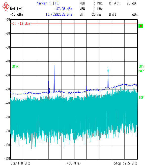
Title: Satellite Tracking People 48270 Comment A: FCC 24 Top channel Date: 14.MAY 2006 16:01:45
