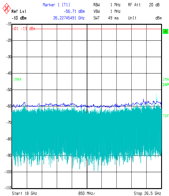
Title: Satellite Tracking People 48270 Comment A: FCC 22 Top channel Date: 14.MAY 2006 17:21:41
