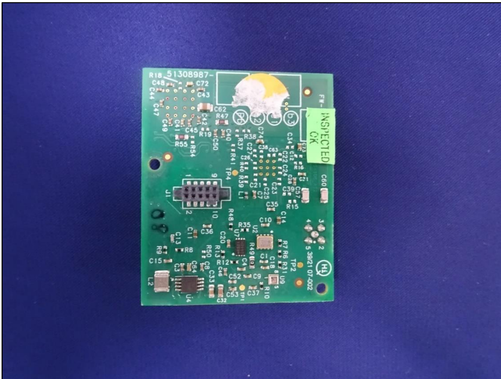
Figure 6: Rear view of RF module
