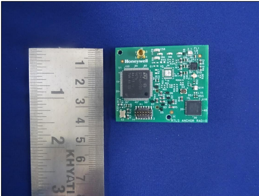
Figure 8: Dimensional view of RF module
