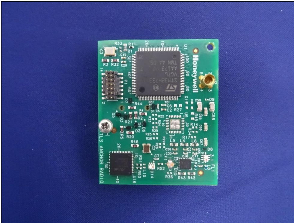
Figure 5: Front view of RF module
