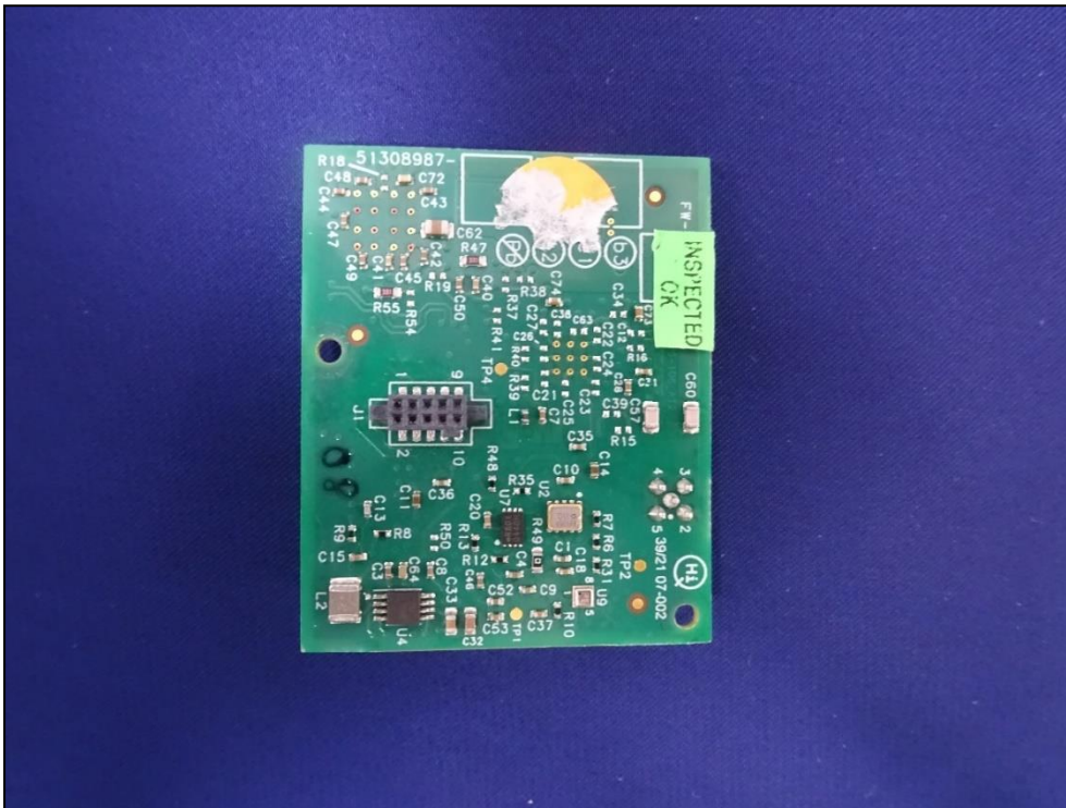
Figure 10: Rear view of RF module (Anchor 1)
