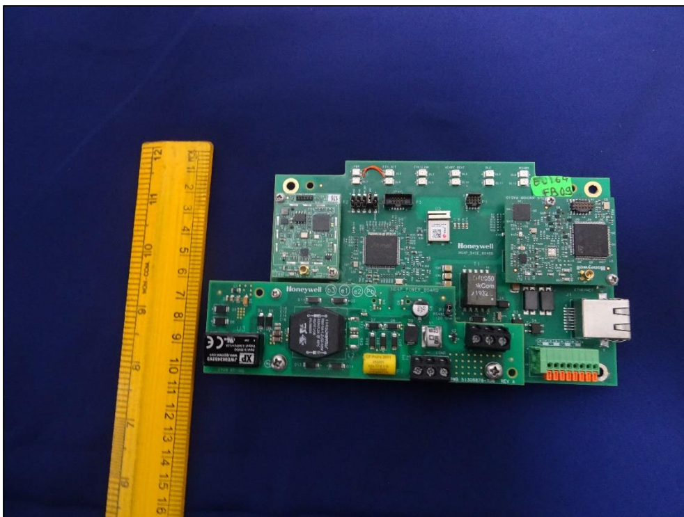
Figure 4: Dimensional view of PCB
