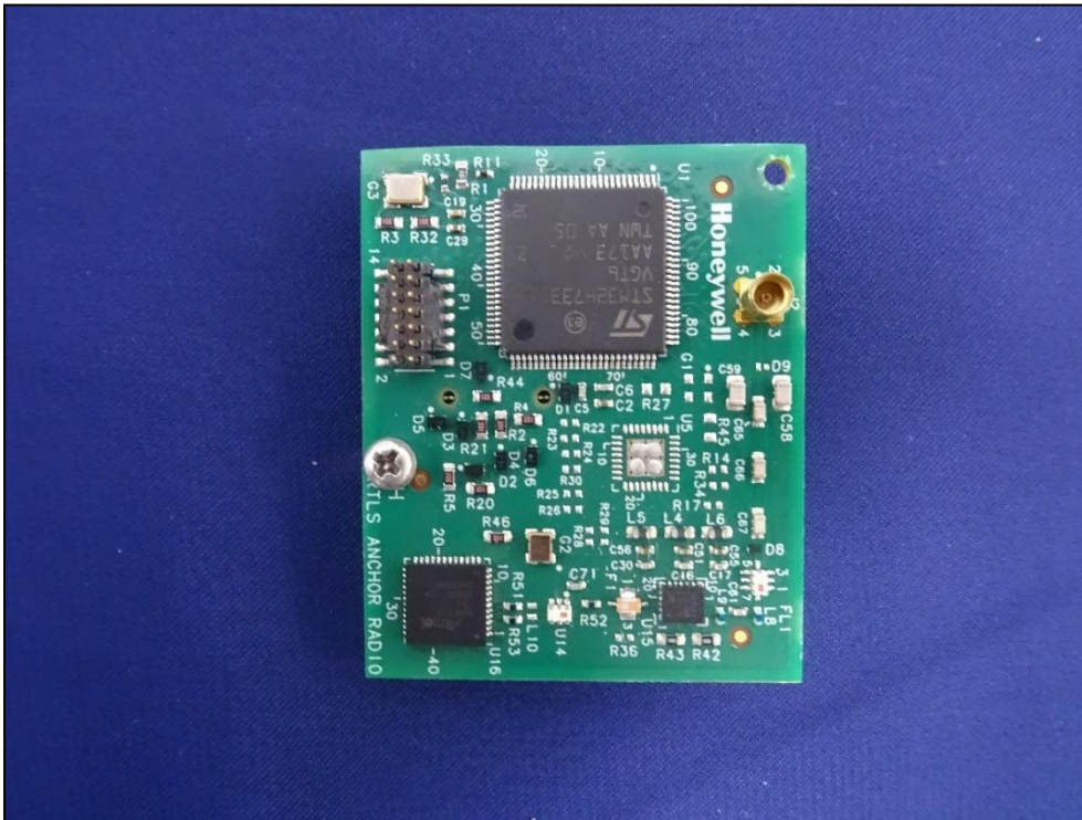
Figure 9: Front view of RF module (Anchor 1)
