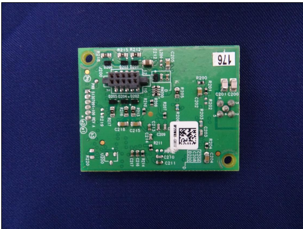
Figure 6: Rear view of RF module (GXR)
