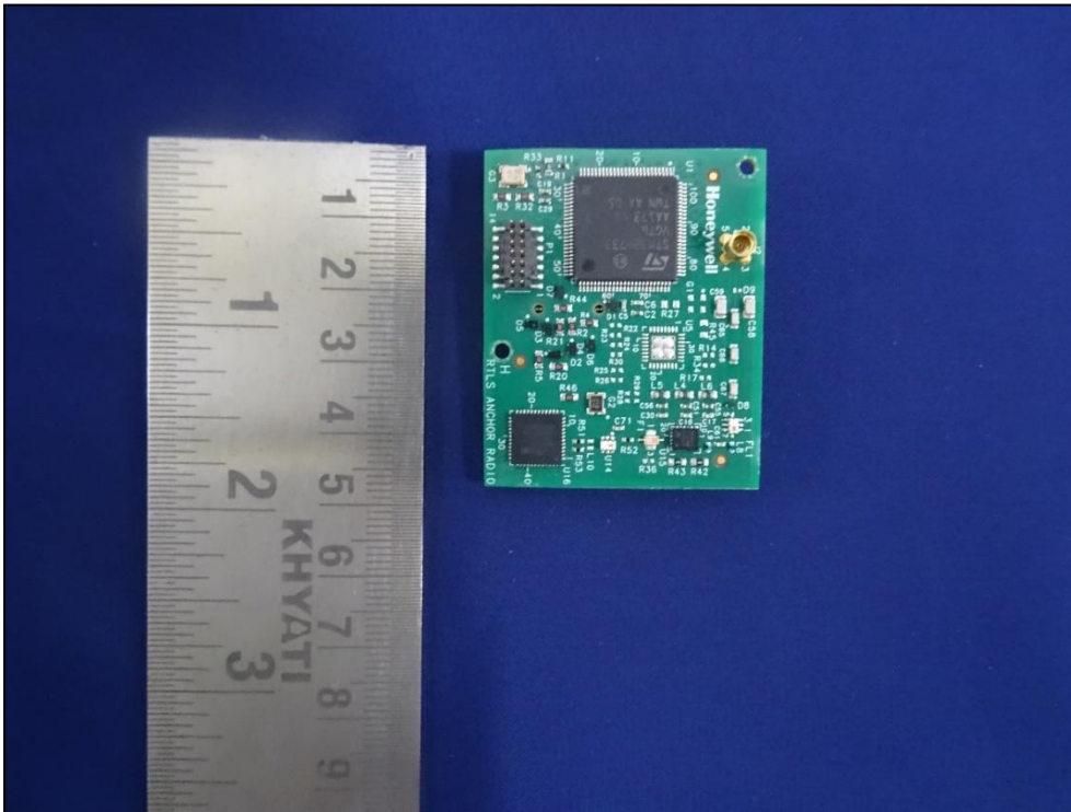
Figure 11: Dimensional view of RF module (Anchor 1)
