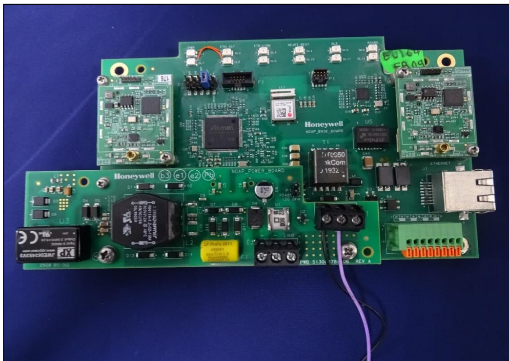
Photo 1: EUT PCB front view
