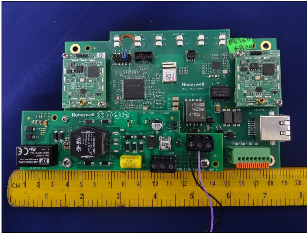
Photo3: PCB Dimension View (Width)
