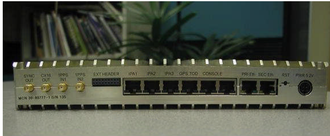
Rear View of Pico 800 MHz BTS
