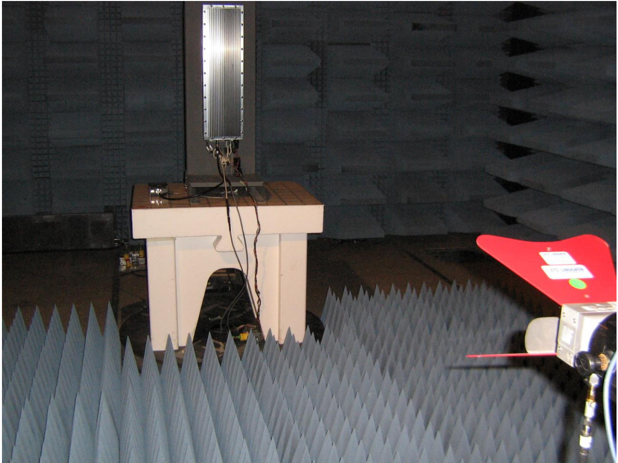
Radiated Emissions Setup above 1 GHz
