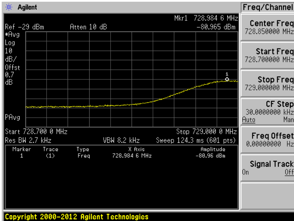
Downlink, Band 12 & 17, GSM 729.2 MHz
