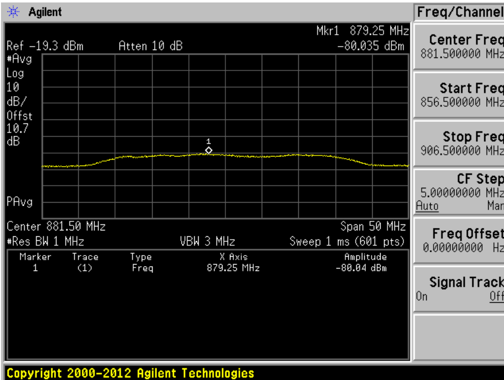
Downlink, Band 5
