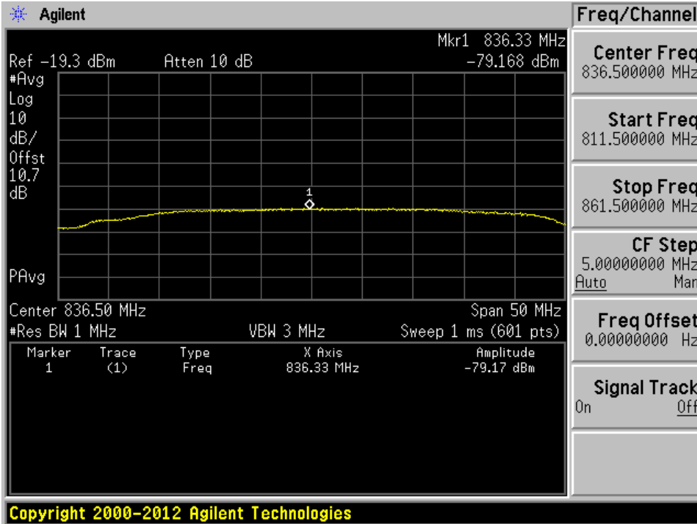
Uplink, Band 5
