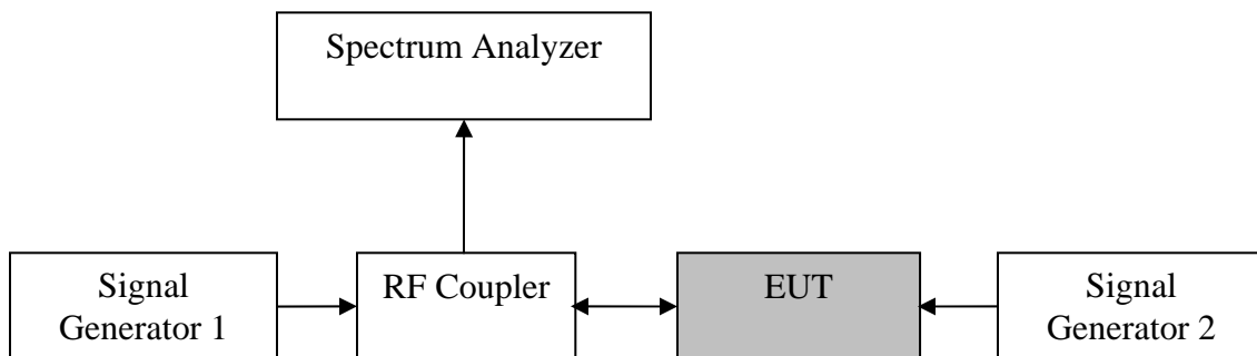
Figure 10: Variable uplink gain test setup
