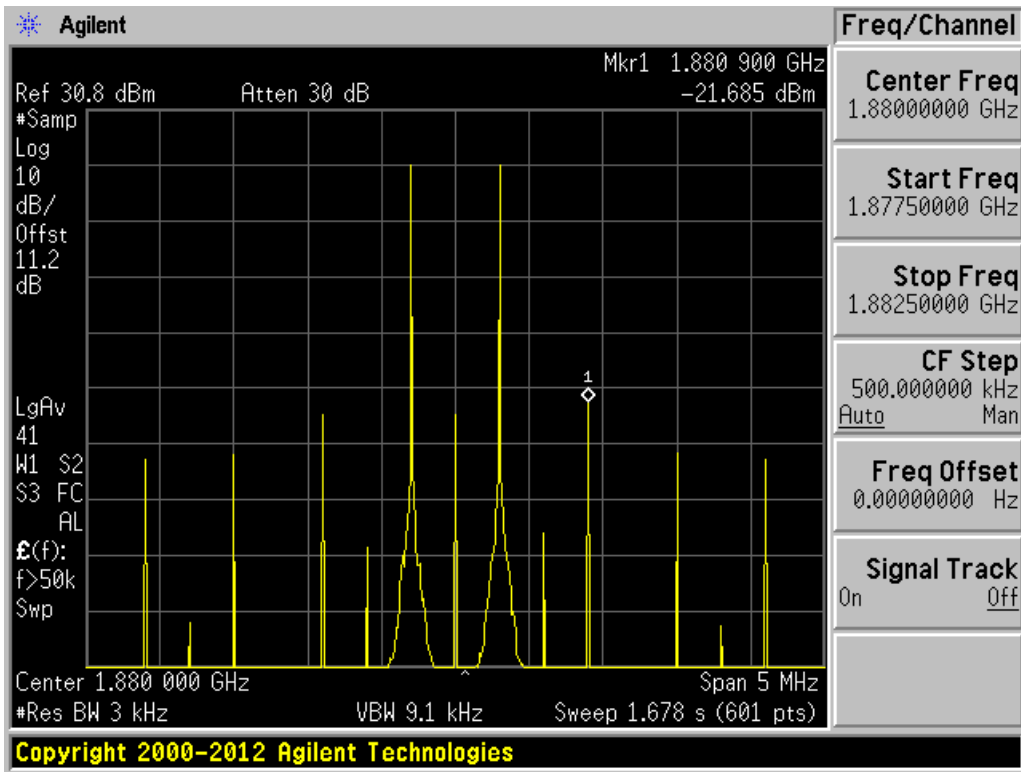
Uplink 1880 MHz.
