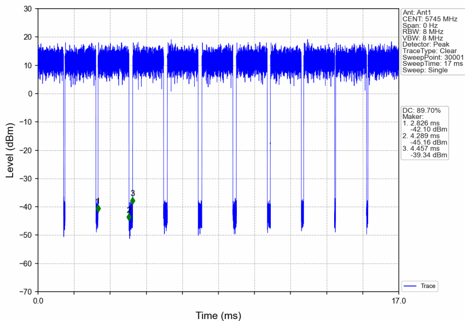
802.11ax(HEW20)_LCH_5745MHz_RU242_Left_Ant1_NTNV
