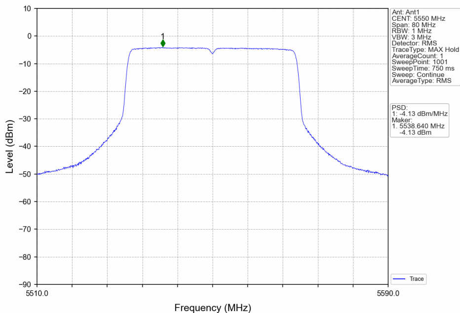
802.11ax(HEW40)_MCH_5550MHz_RU484_Left_Ant1_NTNV
