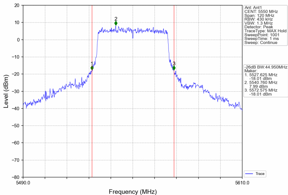
802.11ax(HEW40)_MCH_5550MHz_RU484_Left_Ant1_NTNV
