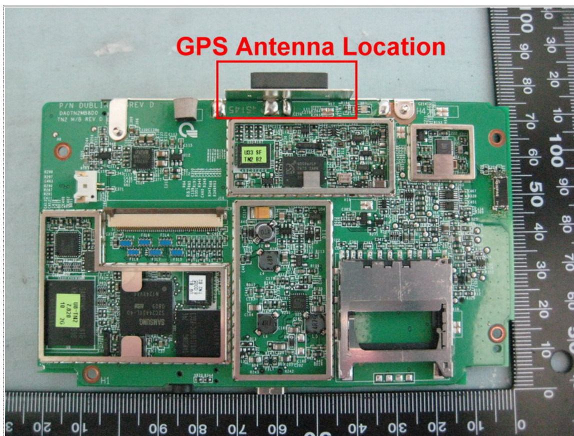
View of GPS Antenna Location
