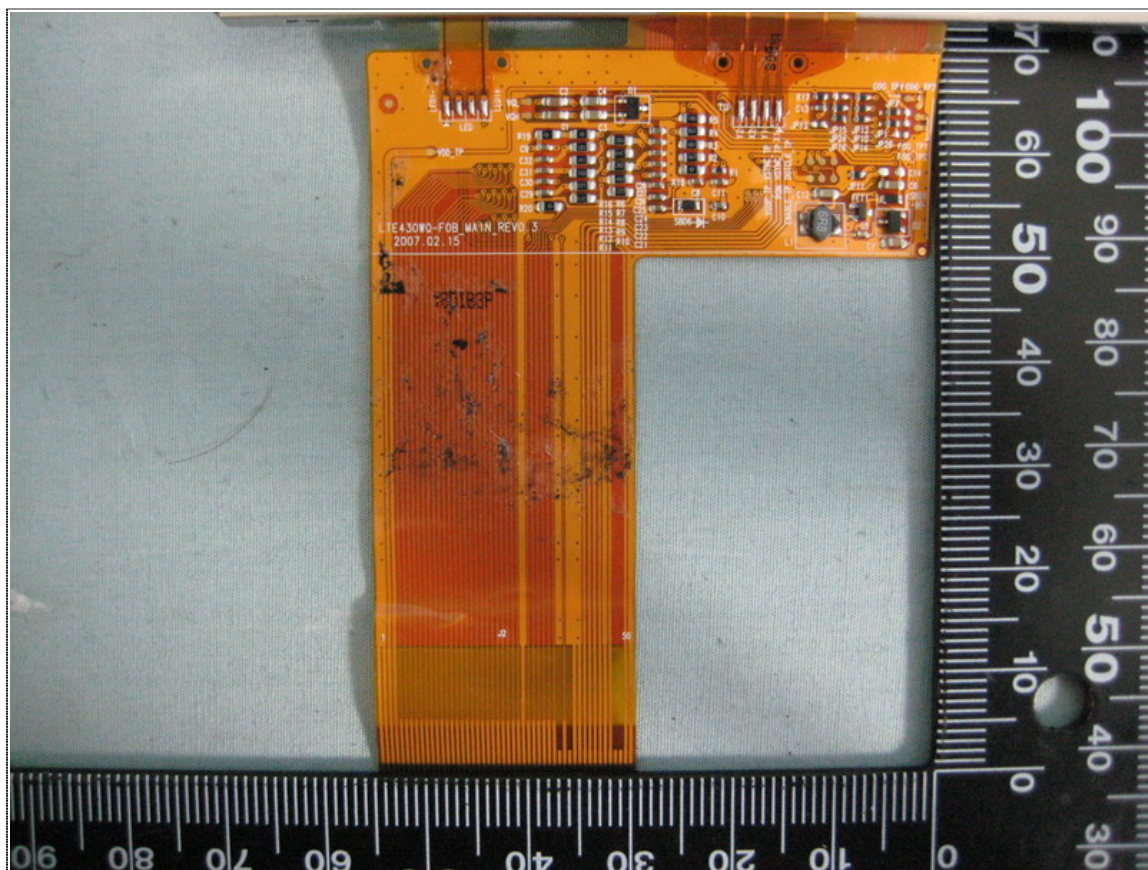
Front View of Panel Main Board
