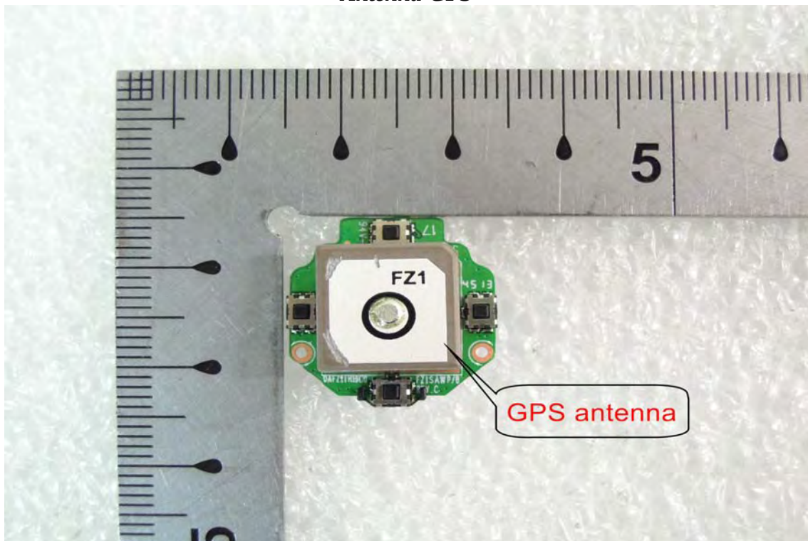
Antenna-GPS
