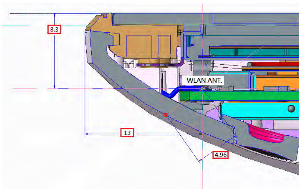
Fig.10 Cross section view
