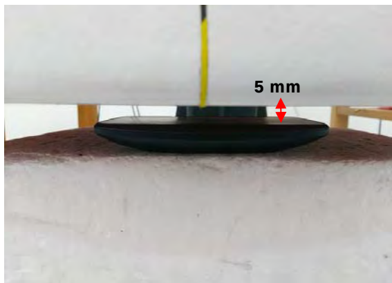
Fig.6 EUT Front side to flat phantom
