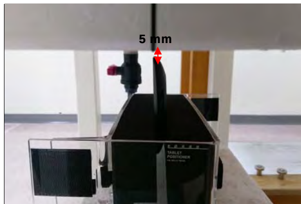
Fig.7 EUT Right side to flat phantom
