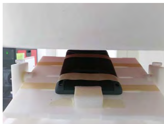
Fig.4 EUT Back side_curve to flat phantom
