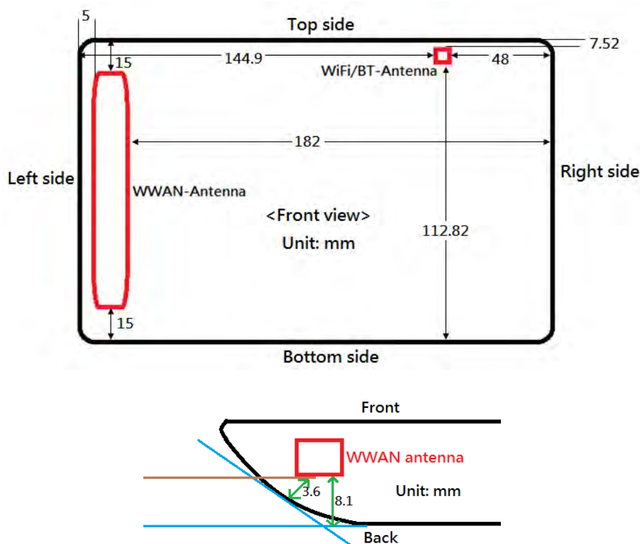
Fig.10 Antenna position of EUT (Front view and Cross section view)
