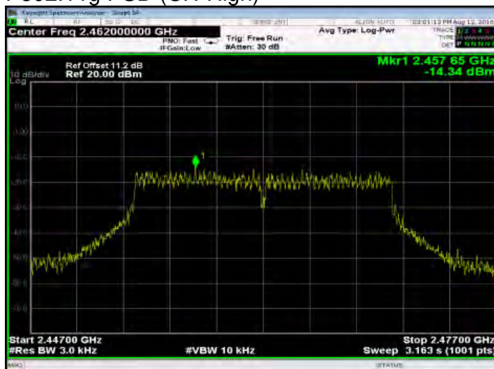
P802.11g PSD (CH-High)
