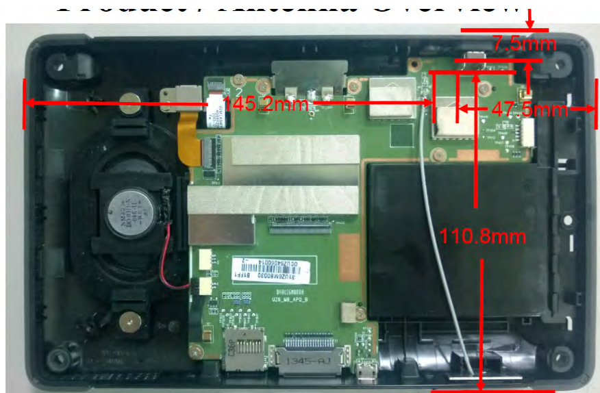
Fig.8 Antenna position of EUT(Back side view)
