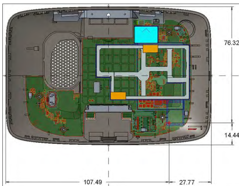
Fig.11 antenna location
