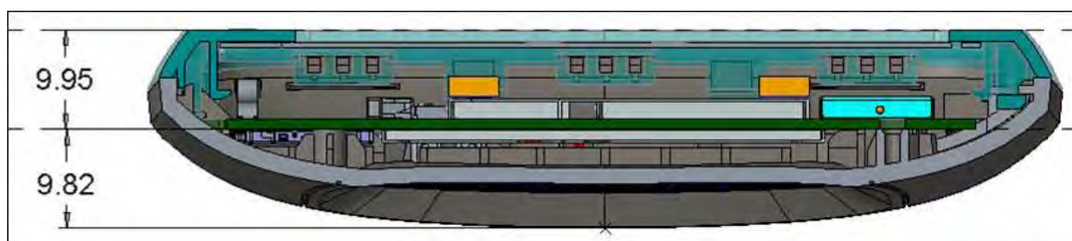
Fig.12 antenna location (edge view)
