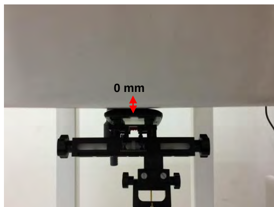
Fig.4 EUT Curve side to flat phantom
