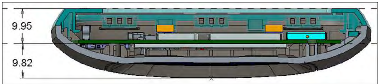
Fig.12 antenna location (edge view)
