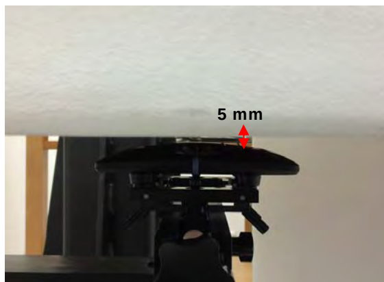
Fig.5 EUT Back side to flat phantom
