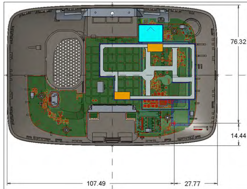
Fig.11 antenna location
