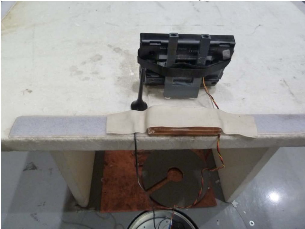
Photo 2: 30-1000MHz Setup
