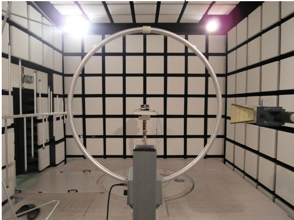
Photo 8: <30MHz Setup
