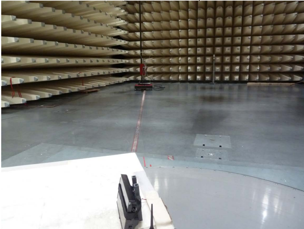
Photo 2: 30-1000MHz Setup
