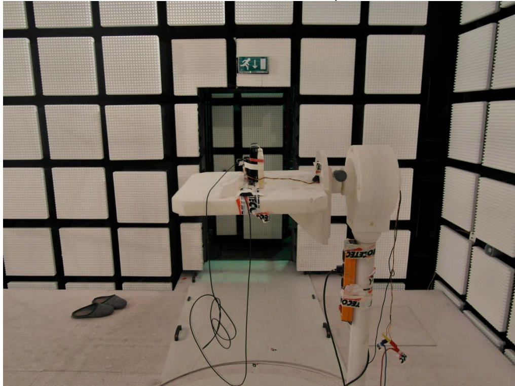
Photo 6: 1-12.75GHz Setup
