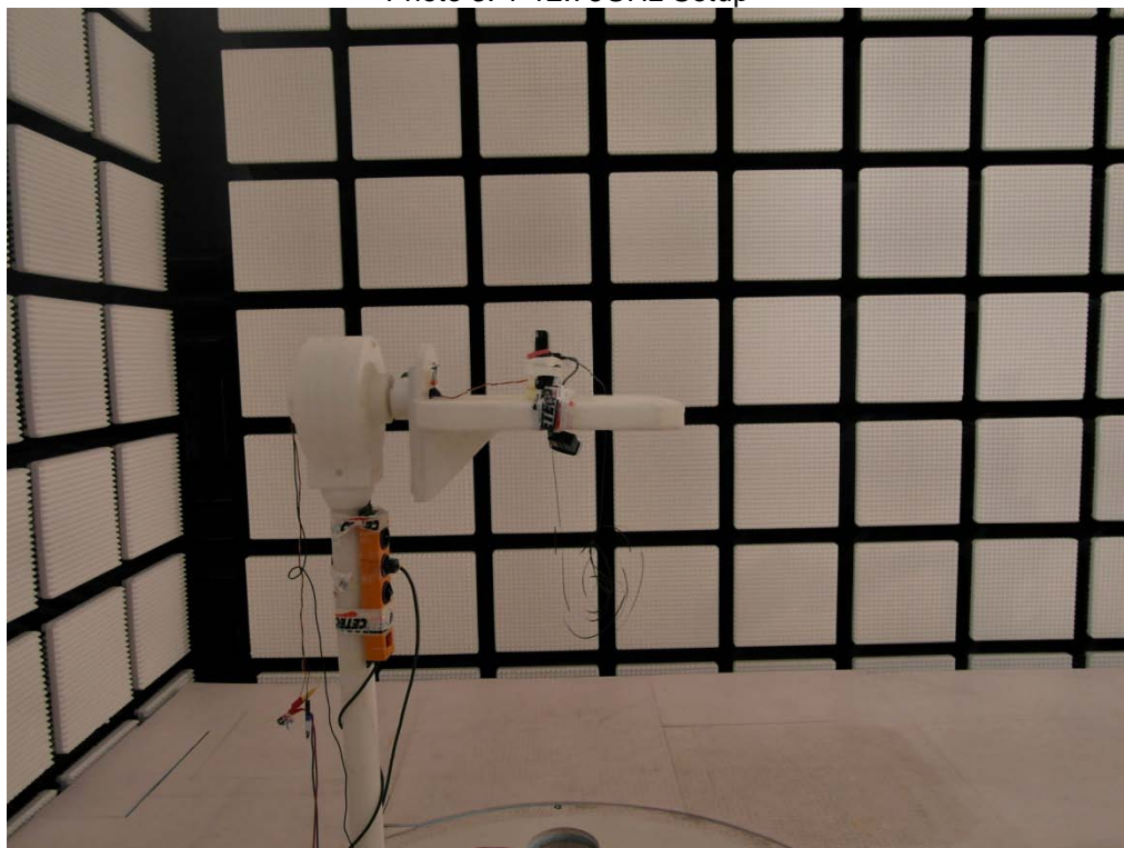
Photo 4: 1-12.75GHz Setup
