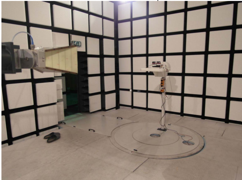
Photo 6: 1-12.75GHz Setup
