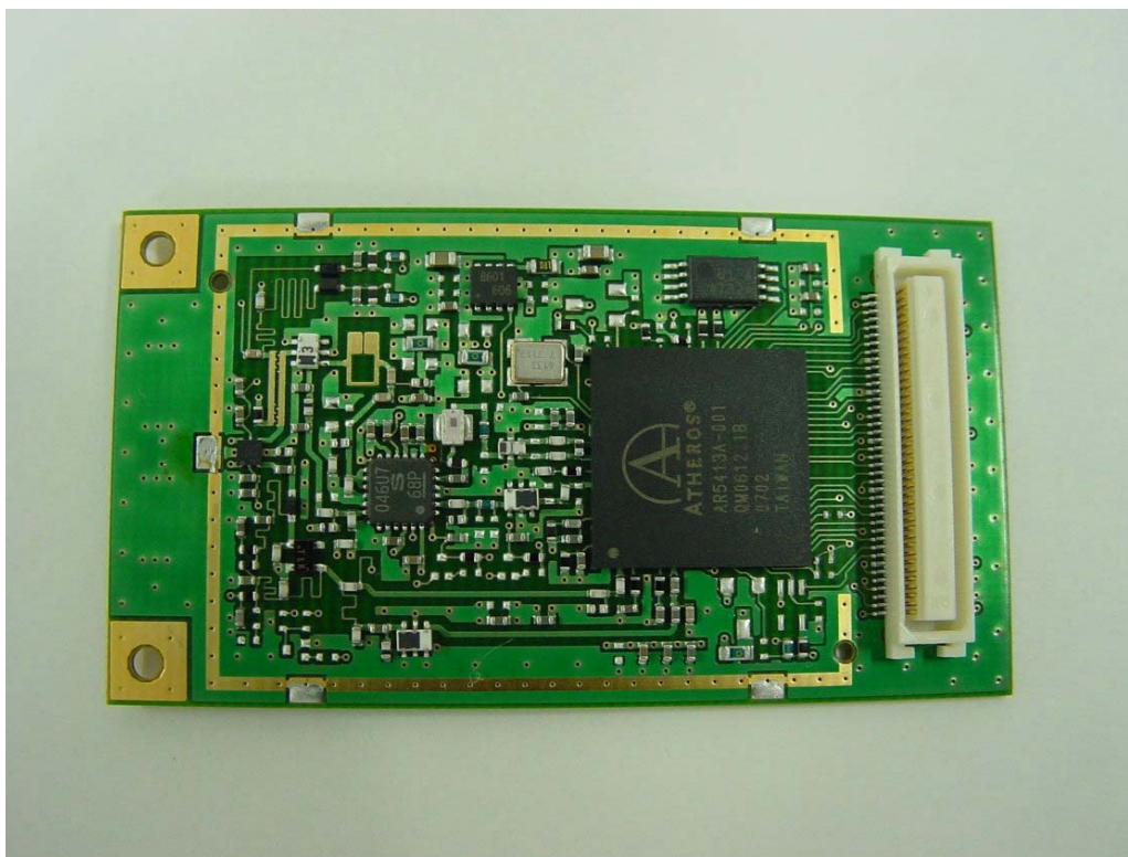
Rear of WLAN Module without Shield
