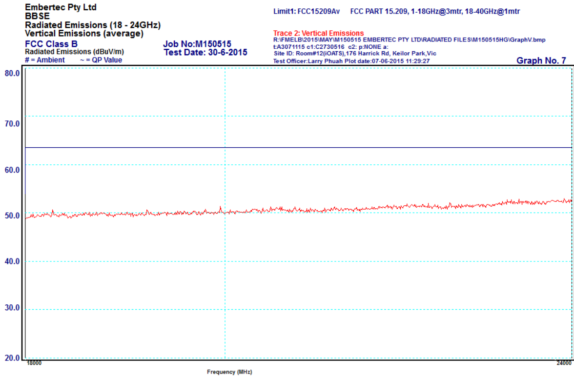
Graph 7: Vertical Polarity (average) 18 – 24 GHz
