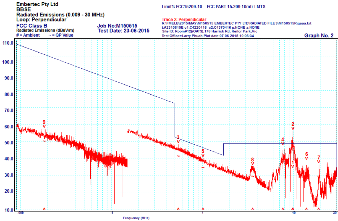
Graph 2: Loop: Perpendicular 9 kHz – 30 MHz
