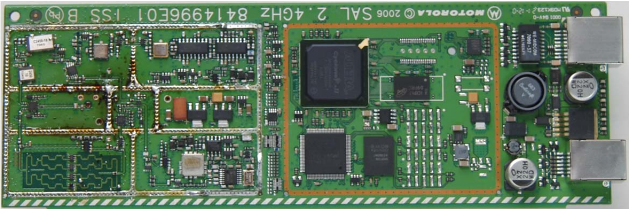
View of the Stinger PCB – Component Side with RF Shield Removed
