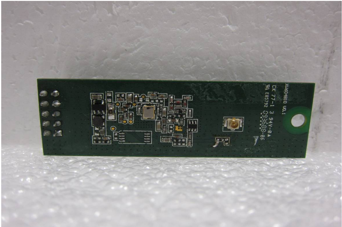
Internal of EUT – 8 (WLAN Antenna)
