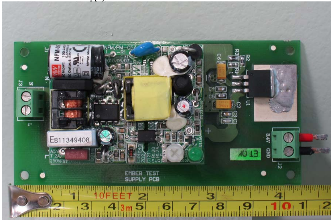
Front Module Power Supply
