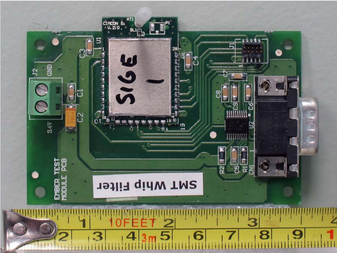
Front – Fixed Antenna
