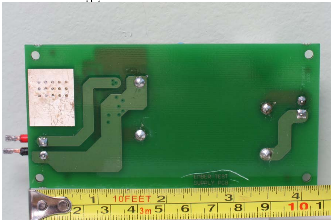
Rear Module Power supply
