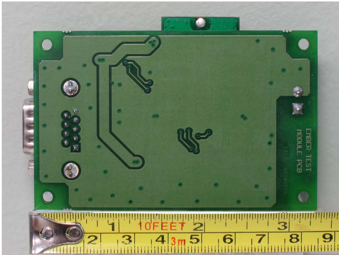
Rear – UFL Antenna
