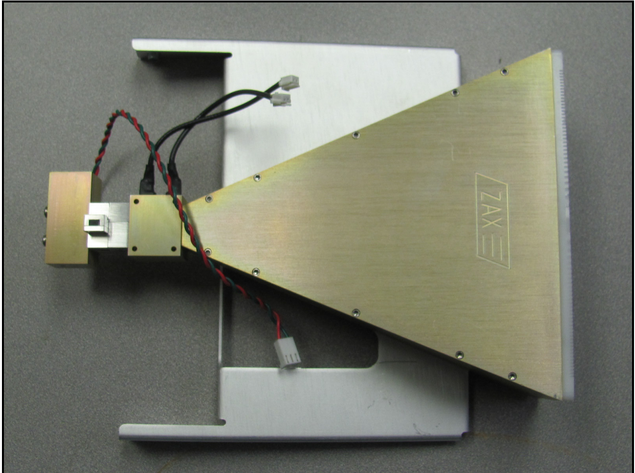
Photograph 16: Horn Bottom View
