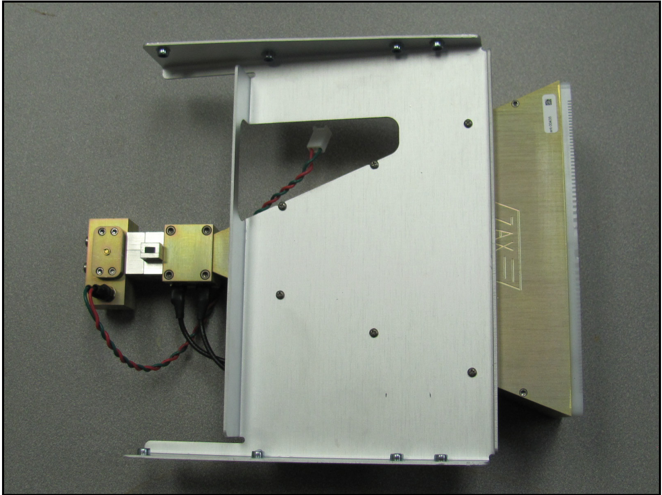
Photograph 15: Horn Top View
