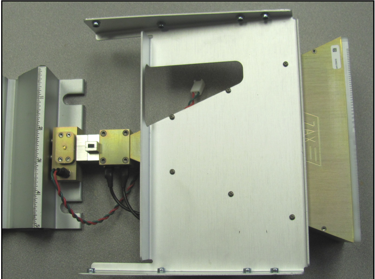
Photograph 17: Scale, Microwave Top View and Horn Top View
