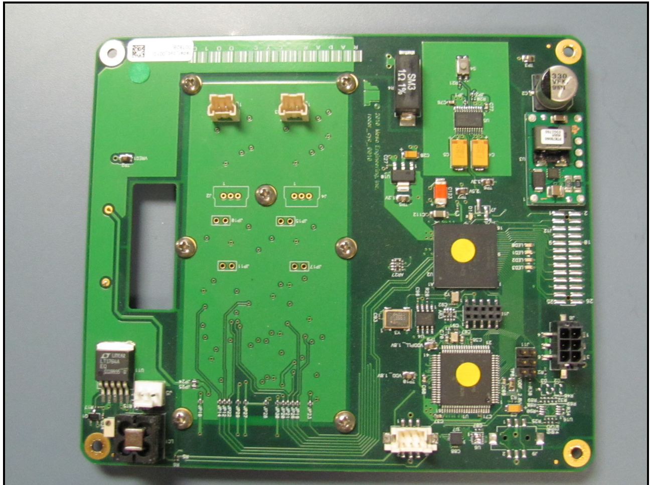
Photograph 10: PCB Top View
