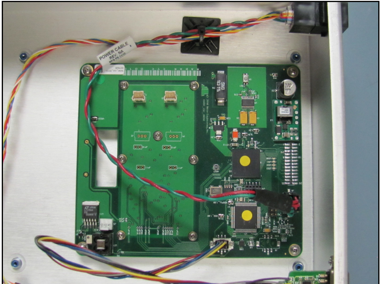
Photograph 9: Assembly PCB
