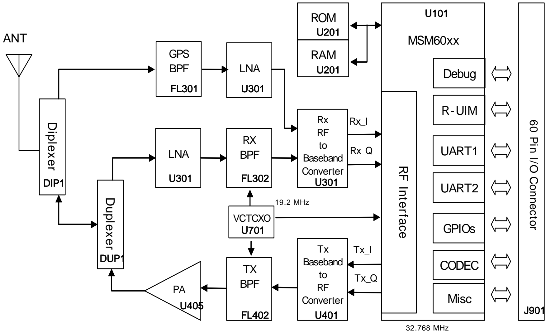
BCM-860S Block Diagram
