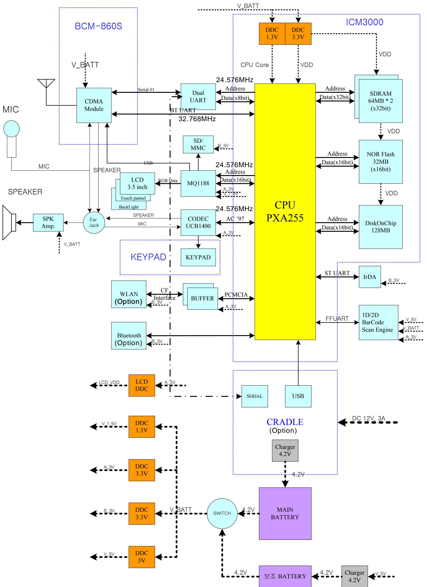
MC3000 BLOCK DIAGRAM
