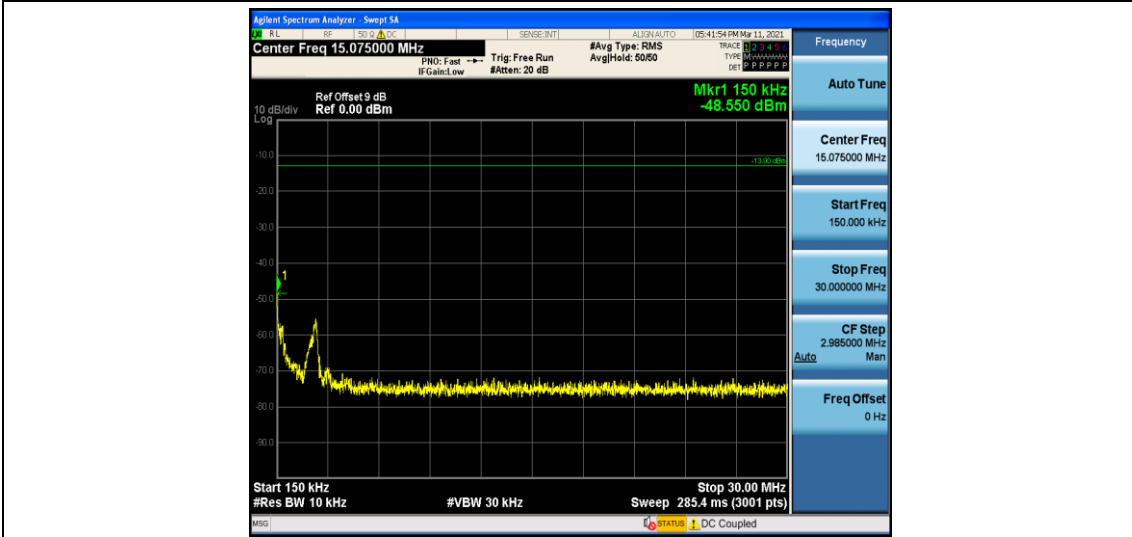
Band 71_5MHz_16QAM_133297_1RB#0
