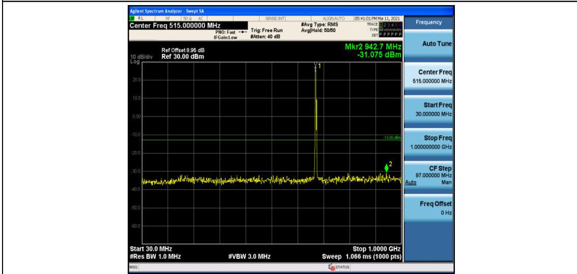
Band 71_5MHz_QPSK_133297_1RB#0
