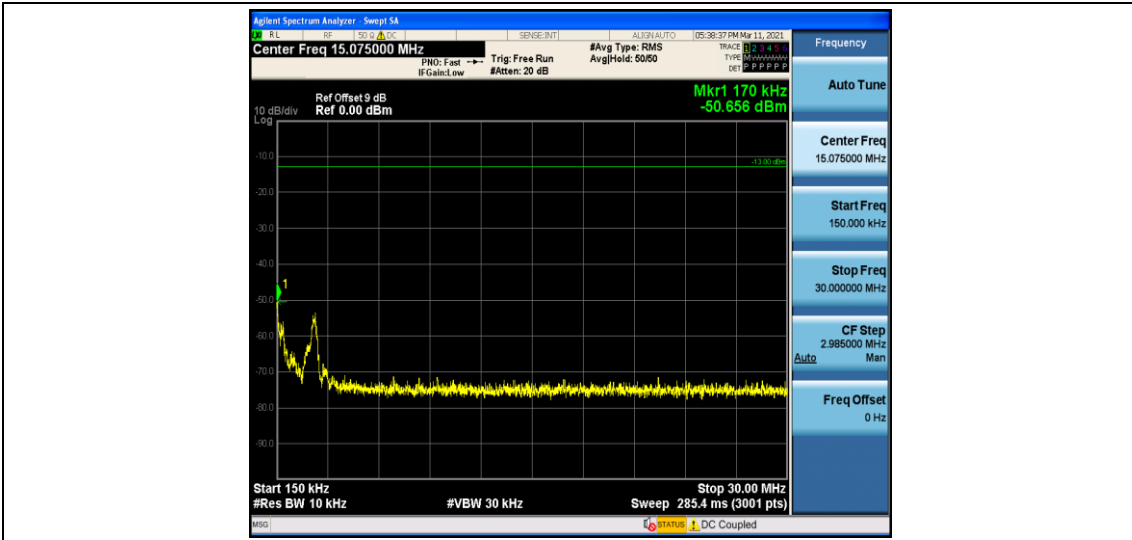
Band 71_5MHz_QPSK_133147_1RB#0
