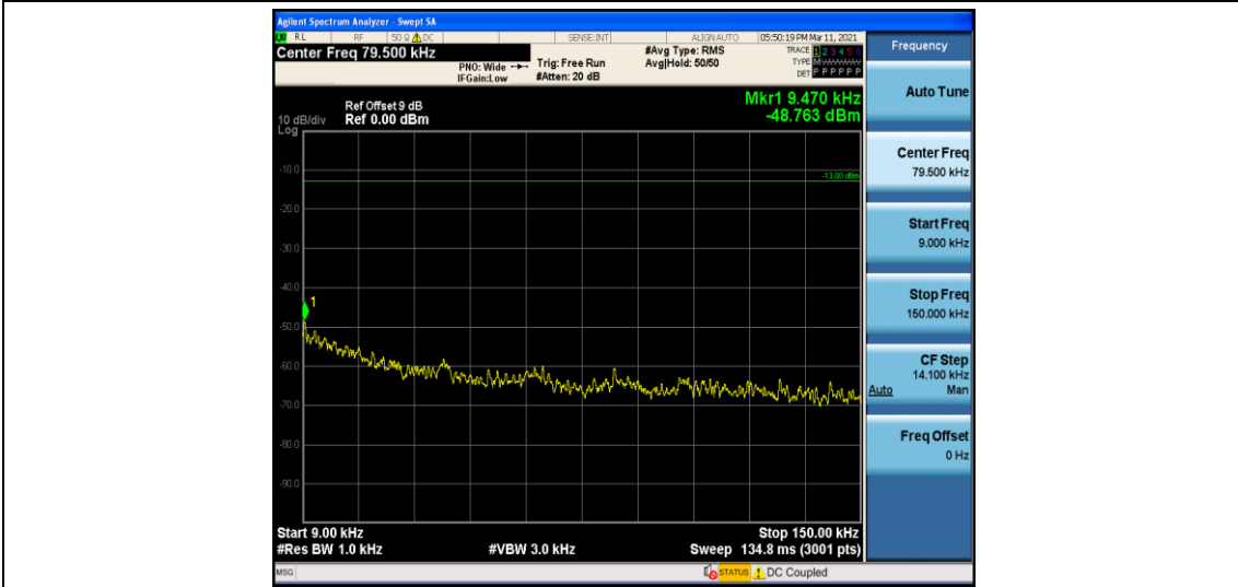
Band 71_10MHz_16QAM_133422_1RB#0
