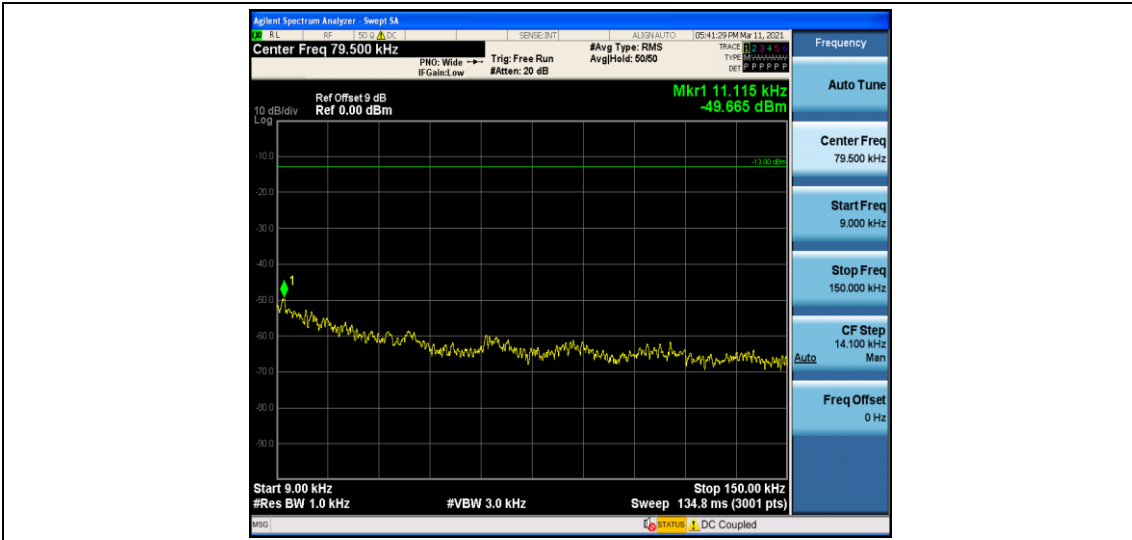
Band 71_5MHz_16QAM_133297_1RB#0
