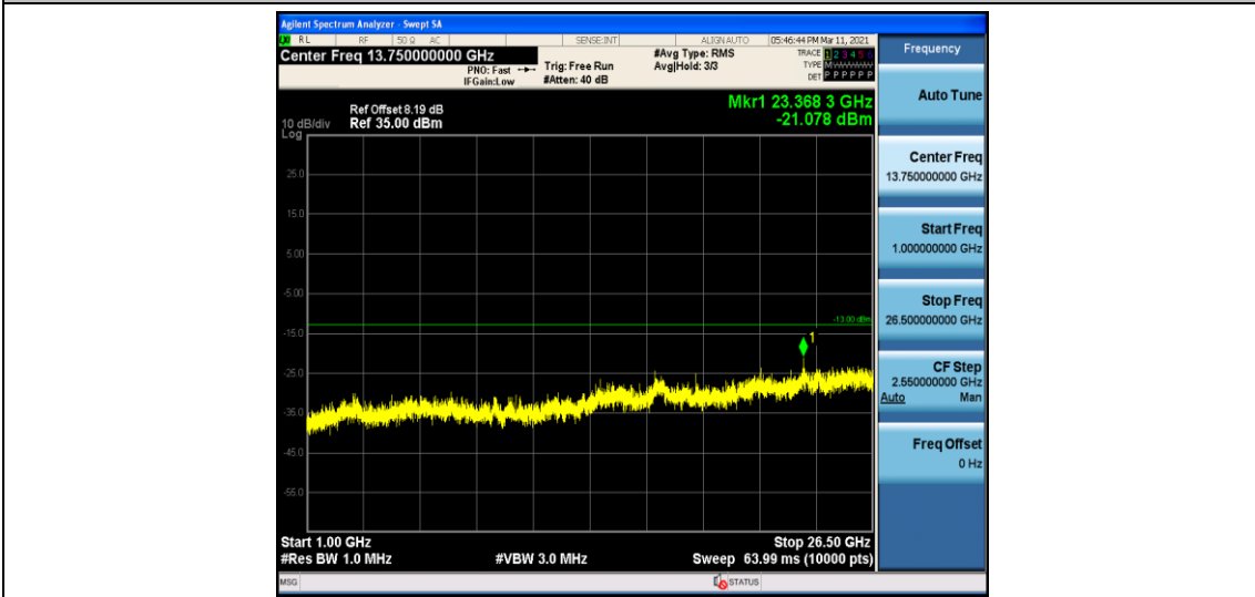
Band 71_10MHz_16QAM_133297_1RB#0
