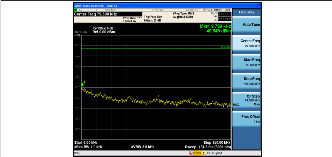
Band66_10MHz_QPSK_132622_1RB#0
