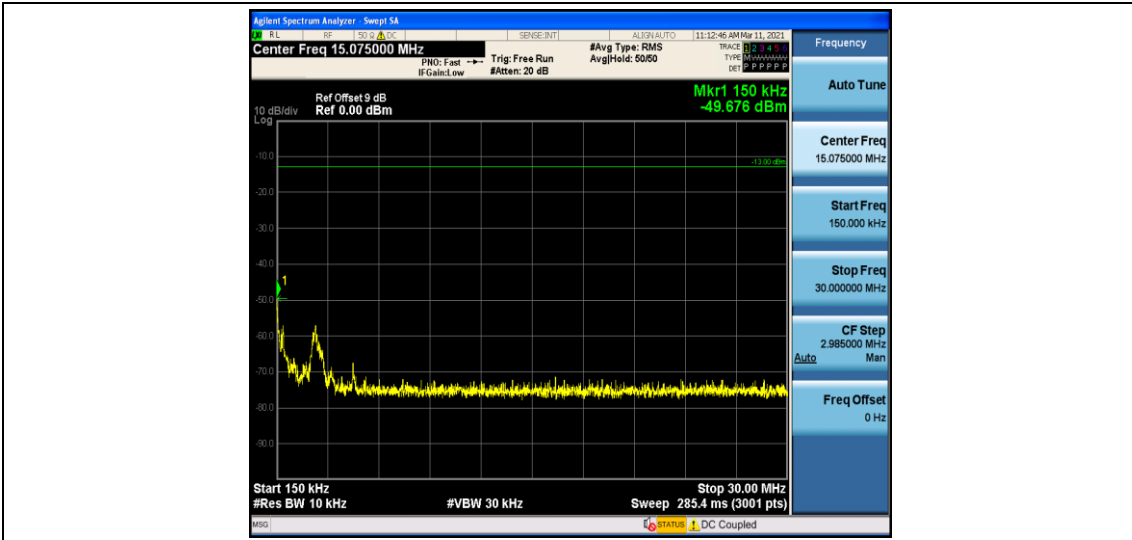
Band66_10MHz_QPSK_132022_1RB#0
