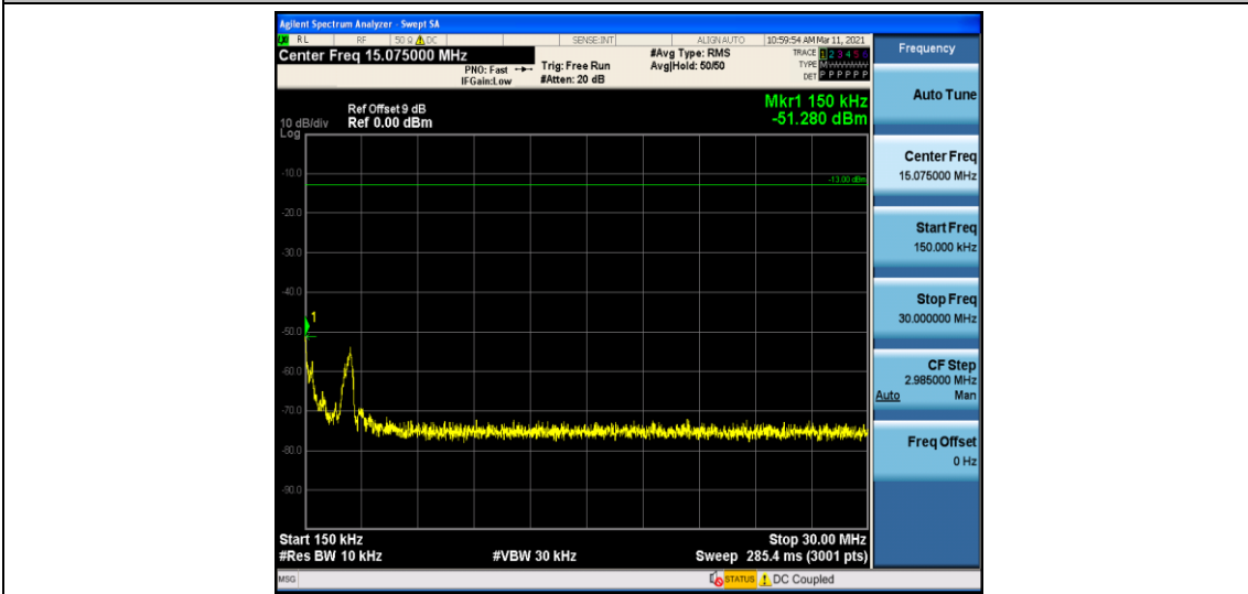
Band66_3MHz_QPSK_132657_1RB#0
