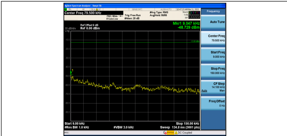
Band66_1.4MHz_QPSK_132322_1RB#0
