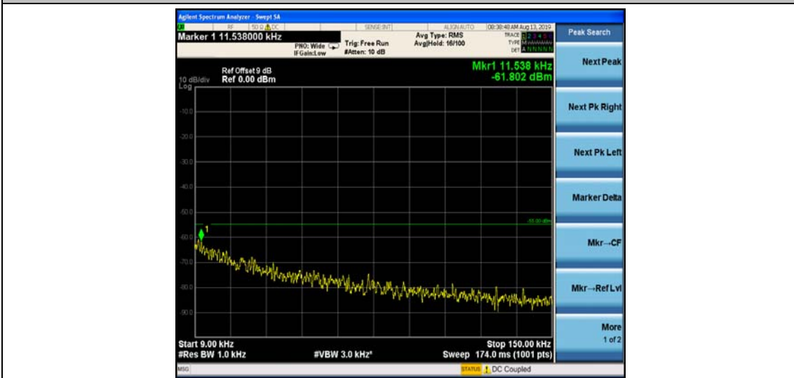
Band41_5MHz_QPSK_40620_1RB#0
