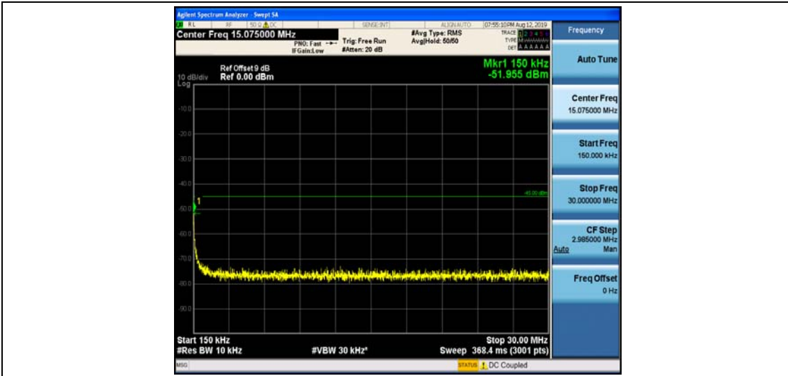
Band41_5MHz_16QAM_39675_1RB#0
