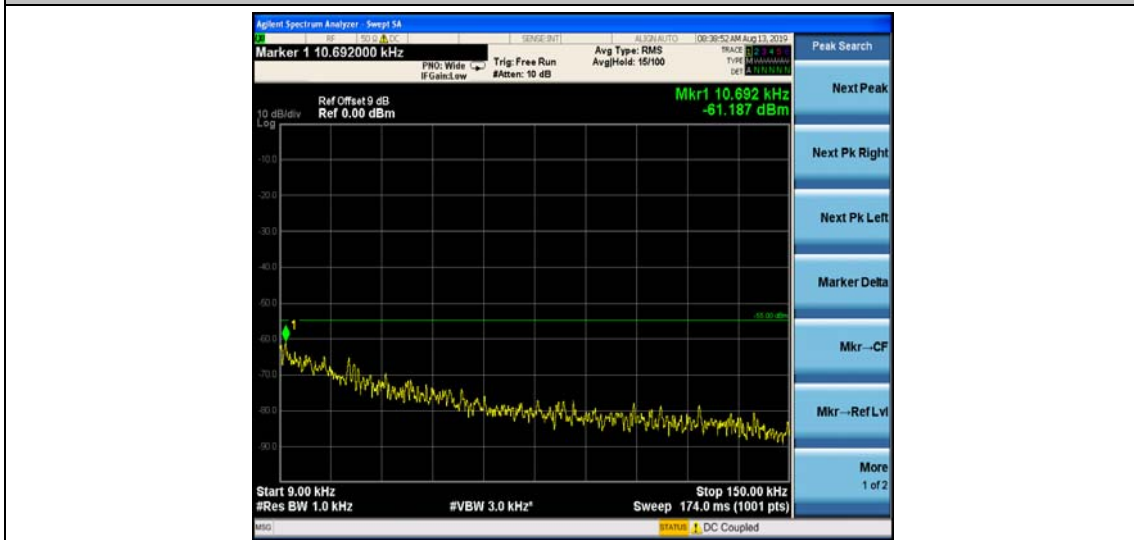
Band41_5MHz_QPSK_41565_1RB#0
