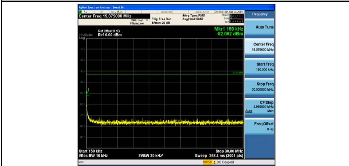
Band25_3MHz_16QAM_24055_1RB#0
