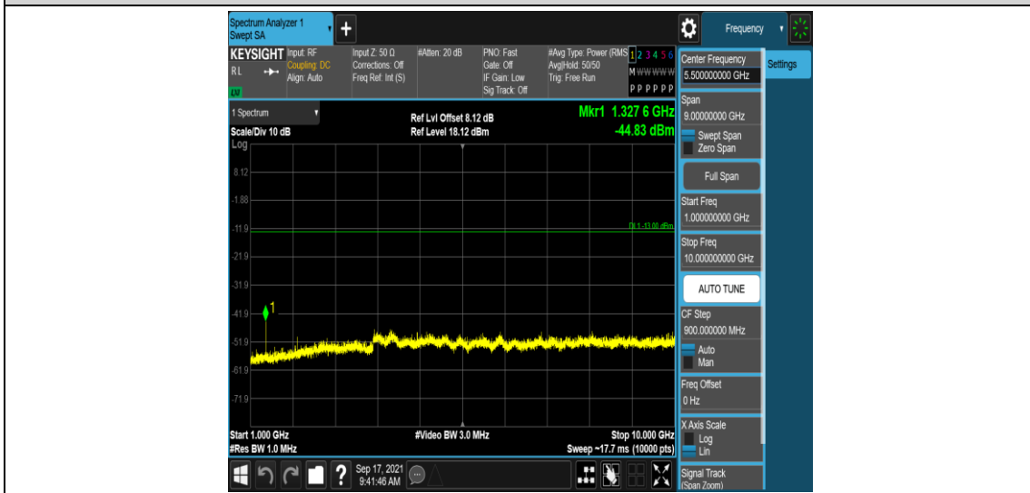
Band71-20MHz-16QAM-133222-1RB#0-Range4:1000~10000MHz
