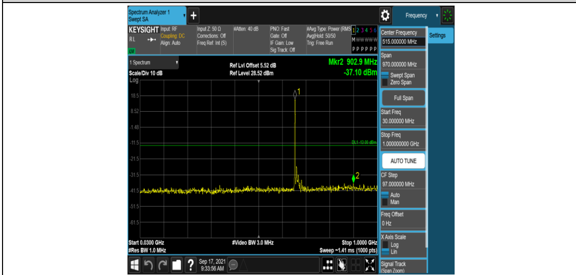
Band71-15MHz-16QAM-133197-1RB#0-Range3:30~1000MHz
