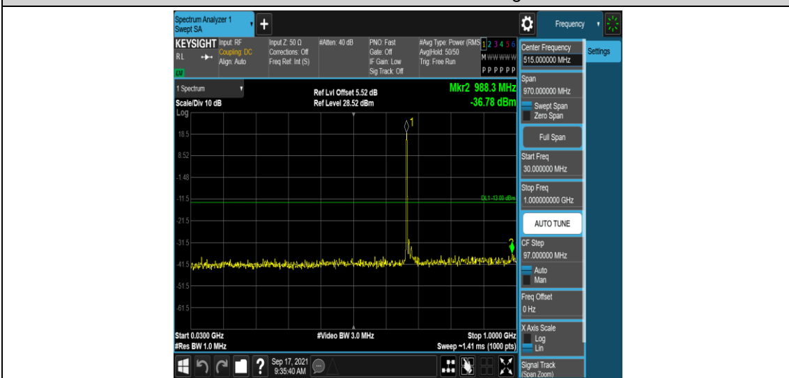
Band71-15MHz-16QAM-133297-1RB#0-Range3:30~1000MHz
