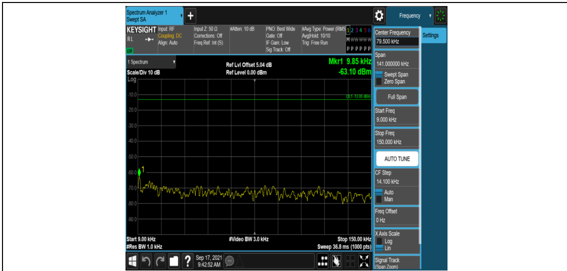
Band71-20MHz-16QAM-133322-1RB#0-Range1:0.009~0.15MHz
