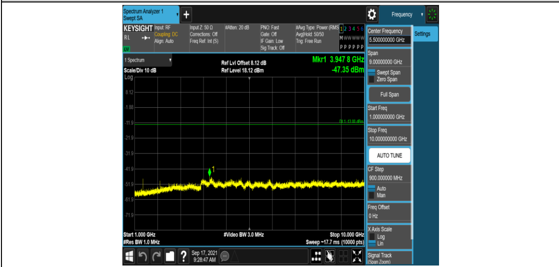
Band71-10MHz-16QAM-133172-1RB#0-Range4:1000~10000MHz
