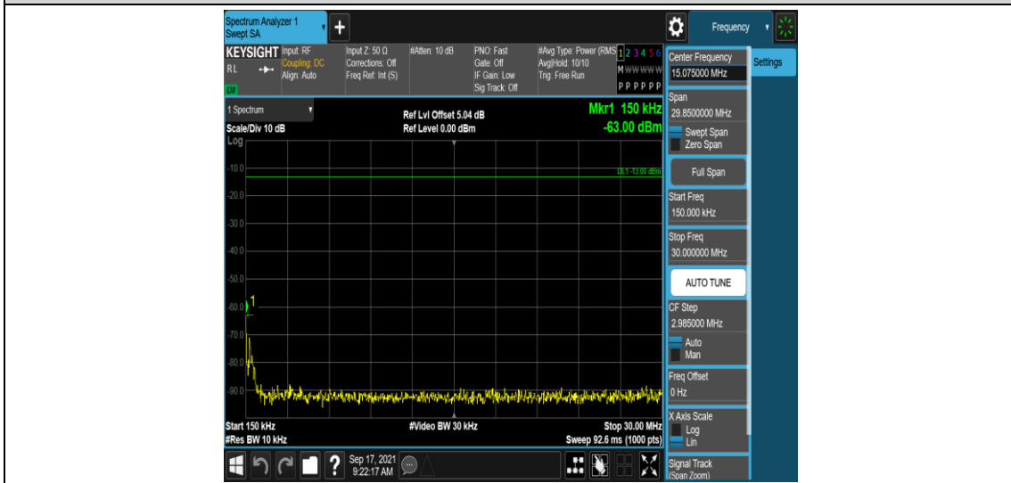
Band71-5MHz-16QAM-133297-1RB#0-Range2:0.15~30MHz
