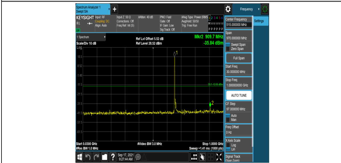
Band71-10MHz-QPSK-133172-1RB#0-Range3:30~1000MHz
