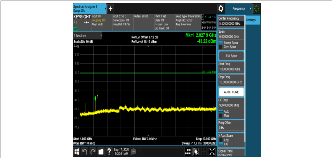
Band71-10MHz-16QAM-133297-1RB#0-Range4:1000~10000MHz
