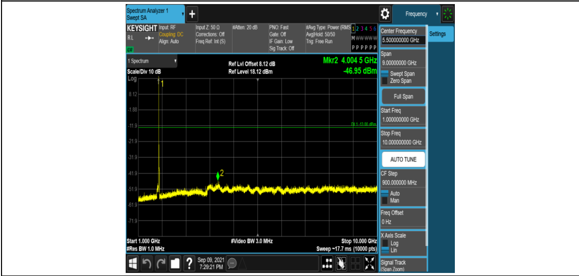
Band66-15MHz-QPSK-132597-1RB#0-Range4:1000~10000MHz
