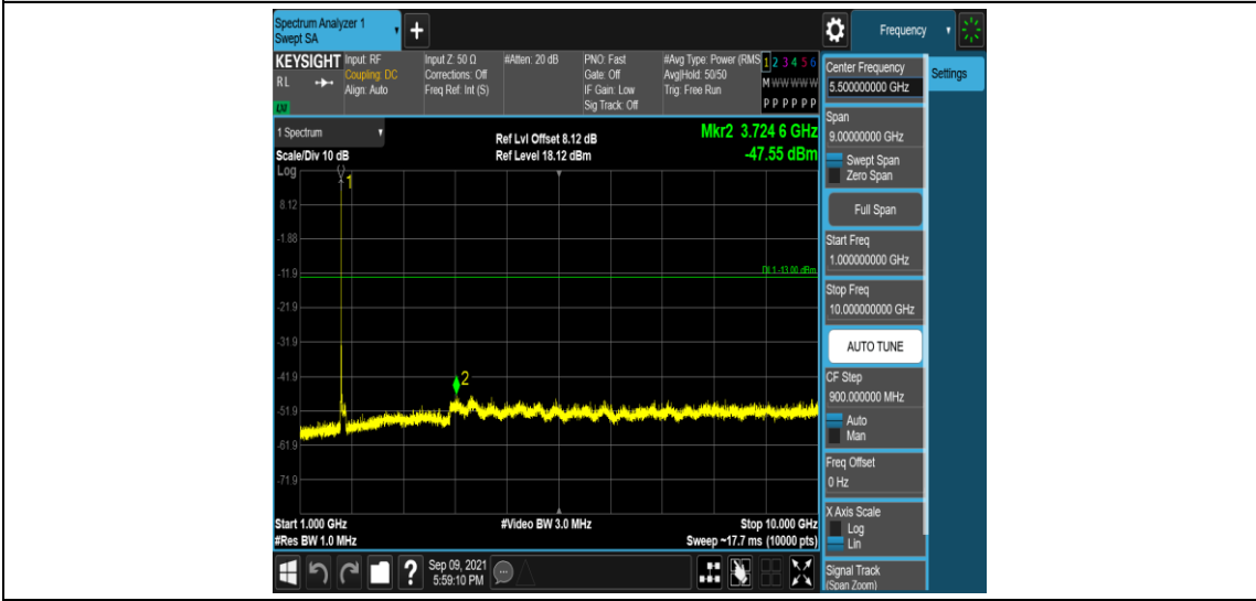
Band66-1.4MHz-16QAM-131979-1RB#0-Range4:1000~10000MHz
