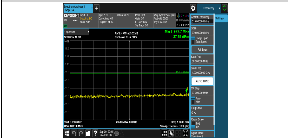
Band66-5MHz-QPSK-131997-1RB#0-Range3:30~1000MHz
