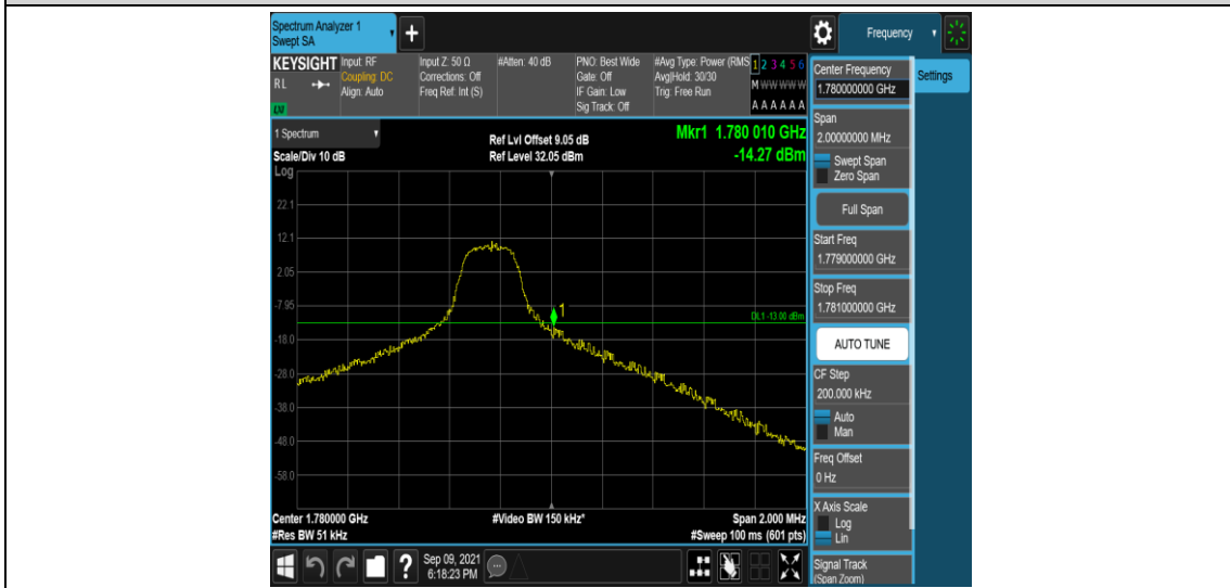
Band66-3MHz-16QAM-132657-1RB#14
