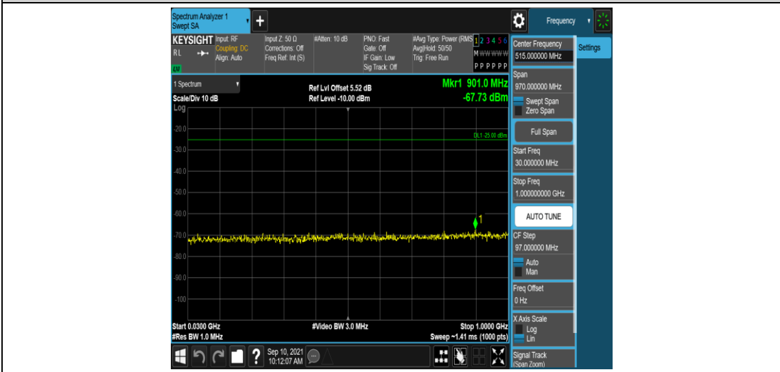
Band41-10MHz-16QAM-40620-1RB#0-Range3:30~1000MHz
