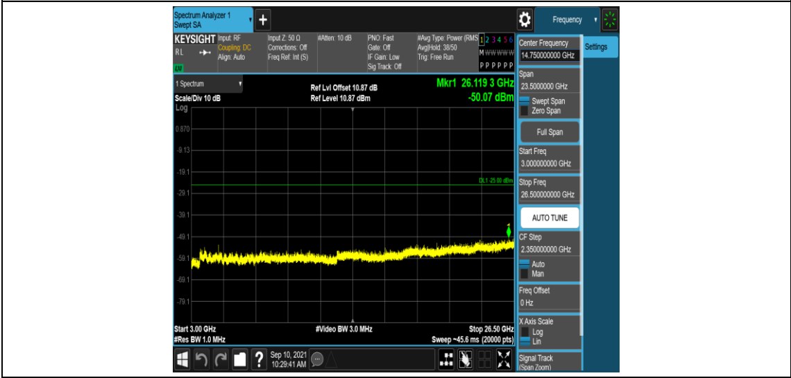
Band41-15MHz-QPSK-39725-1RB#0-Range5:3000~26500MHz
