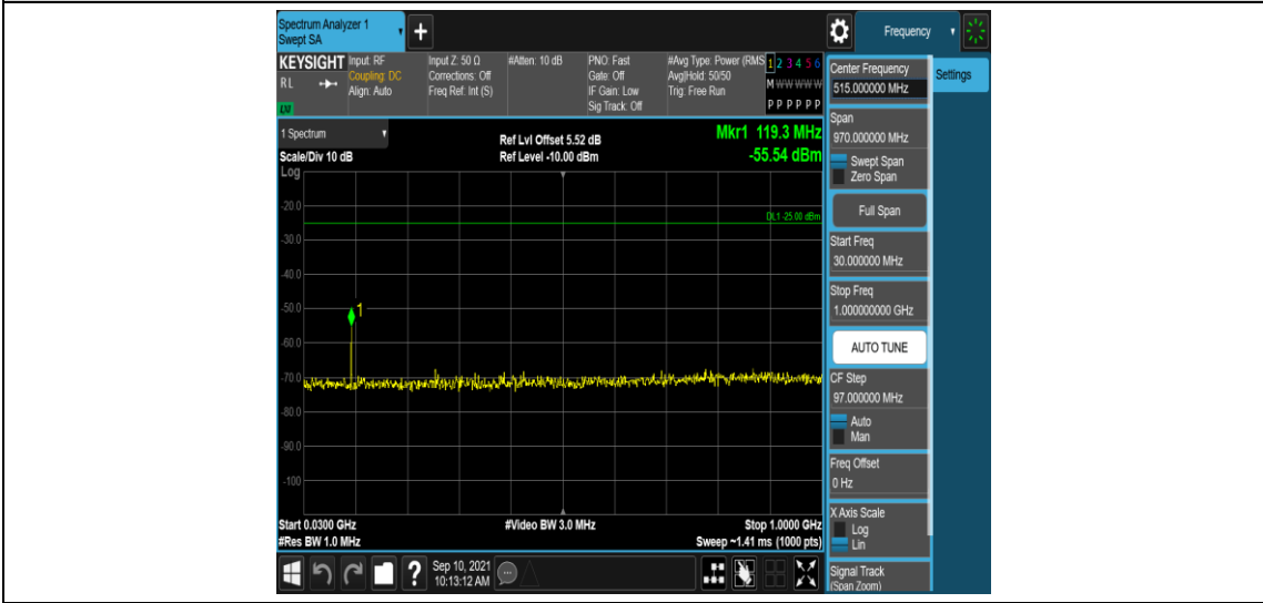
Band41-10MHz-QPSK-41540-1RB#0-Range3:30~1000MHz
