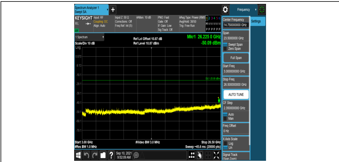
Band41-5MHz-16QAM-41565-1RB#0-Range5:3000~26500MHz
