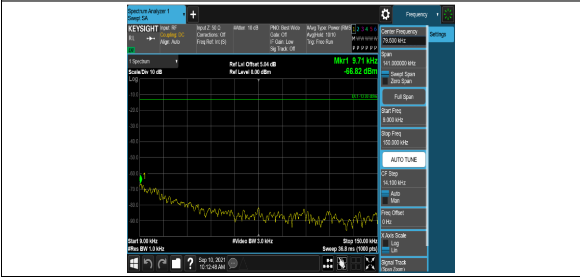
Band41-10MHz-QPSK-41540-1RB#0-Range1:0.009~0.15MHz
