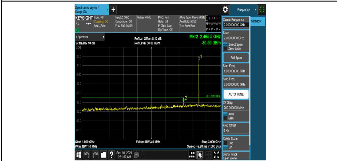
Band41-5MHz-16QAM-41565-1RB#0-Range4:1000~3000MHz
