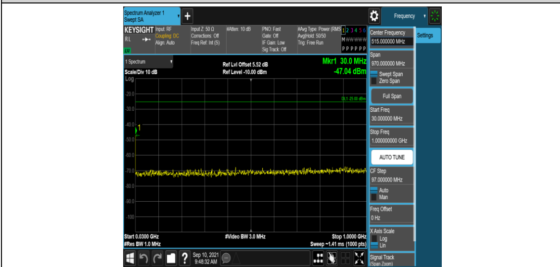
Band41-5MHz-QPSK-40620-1RB#0-Range3:30~1000MHz
