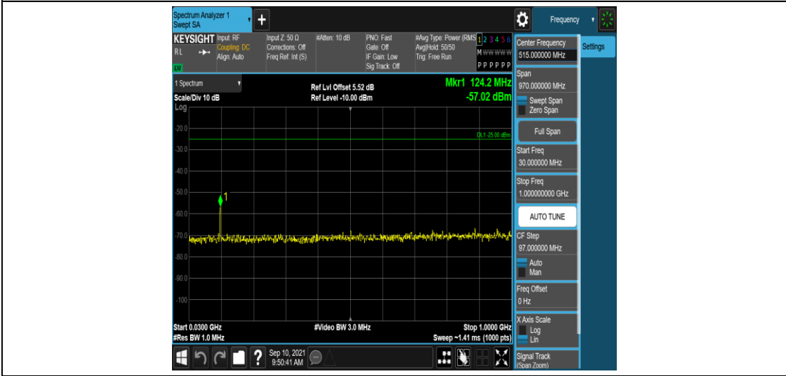
Band41-5MHz-QPSK-41565-1RB#0-Range3:30~1000MHz
