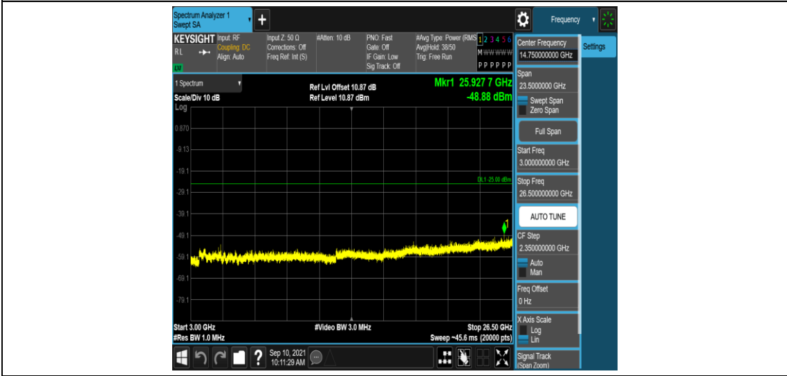
Band41-10MHz-QPSK-40620-1RB#0-Range5:3000~26500MHz
