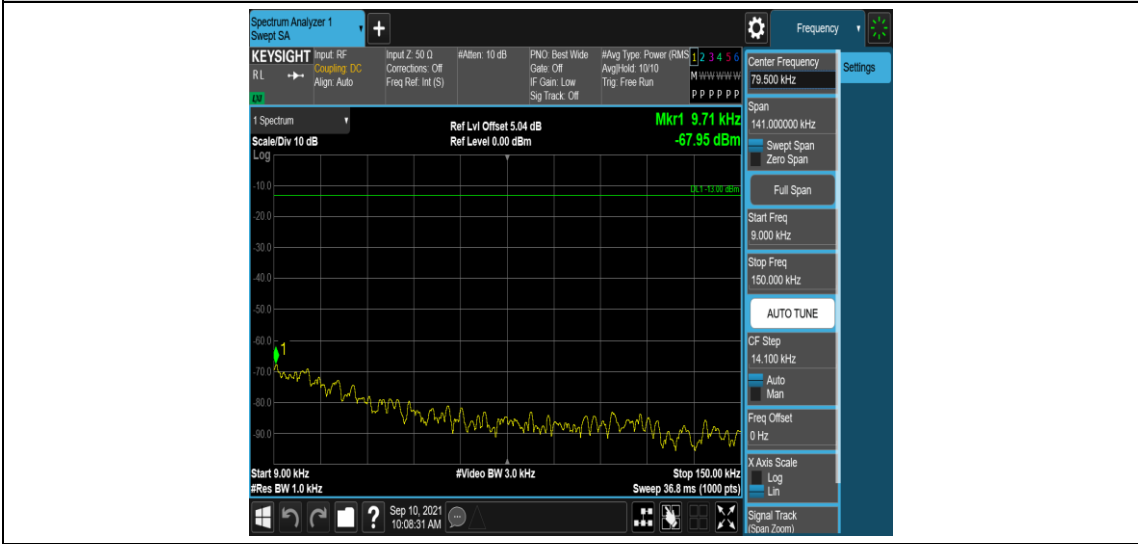
Band41-10MHz-QPSK-39700-1RB#0-Range1:0.009~0.15MHz
