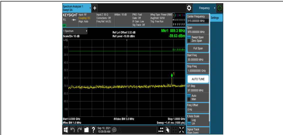
Band41-10MHz-16QAM-39700-1RB#0-Range3:30~1000MHz
