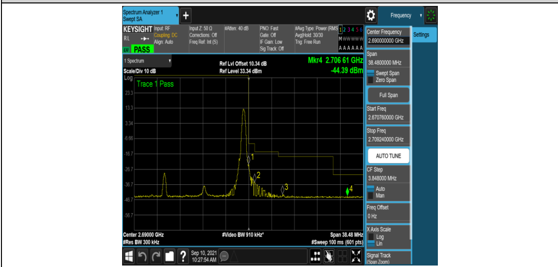
Band41-15MHz-16QAM-41515-1RB#74
