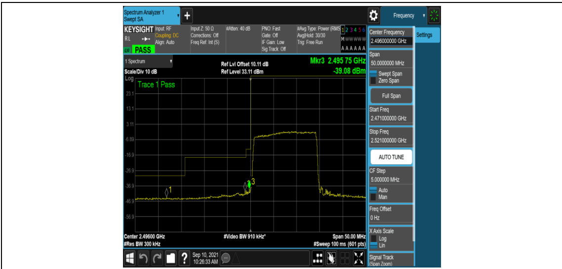
Band41-15MHz-16QAM-39725-75RB#0
