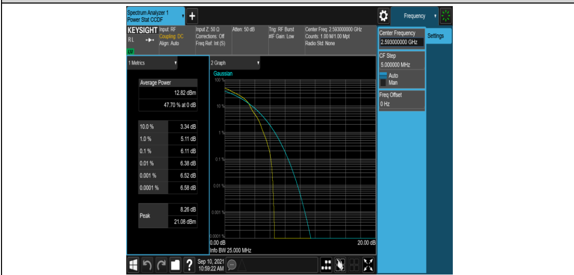
Band41-20MHz-16QAM-40620-1RB#0
