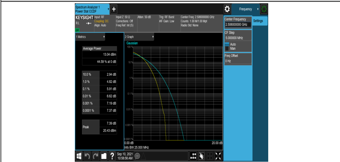
Band41-20MHz-16QAM-39750-100RB#0
