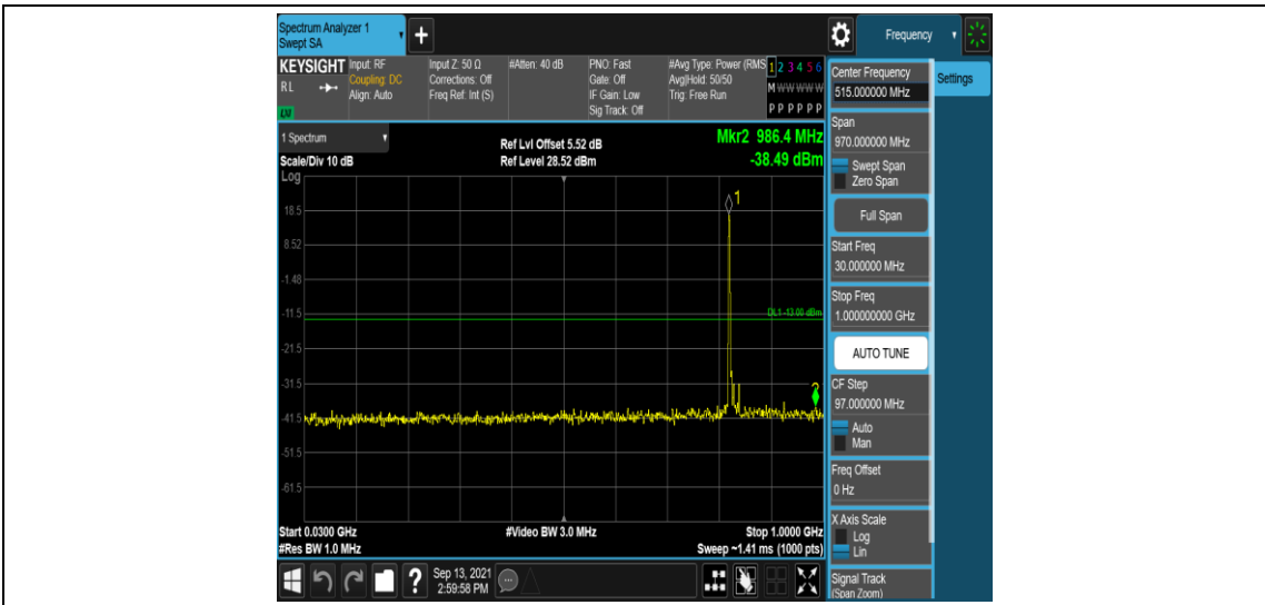
Band26-10MHz-QPSK-26840-1RB#0-Range3:30~1000MHz
