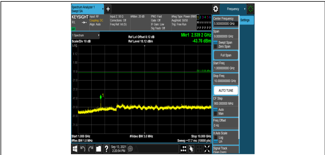
Band26-3MHz-16QAM-27025-1RB#0-Range4:1000~10000MHz
