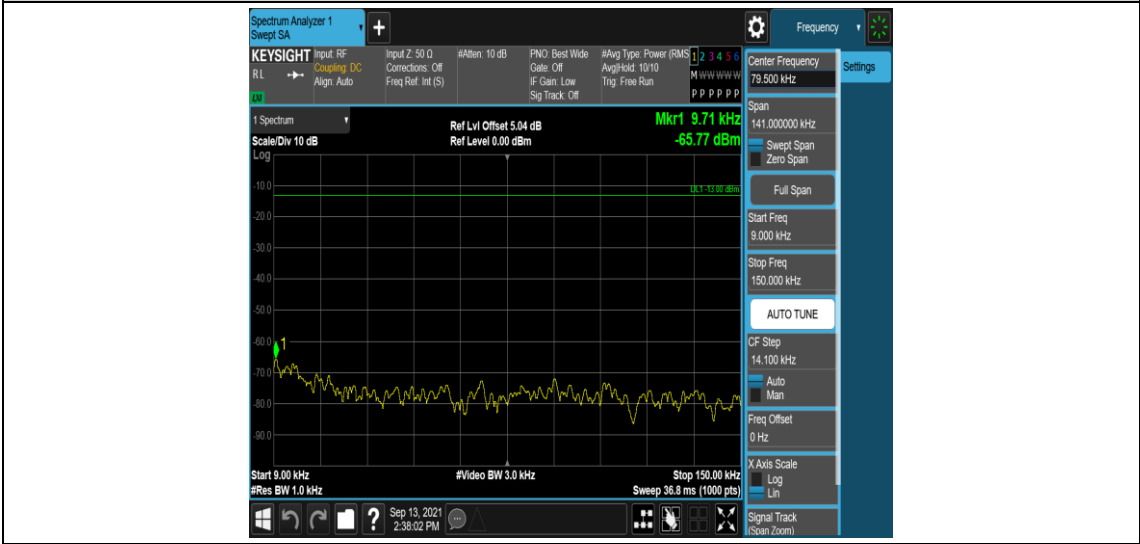
Band26-5MHz-QPSK-26815-1RB#0-Range1:0.009~0.15MHz
