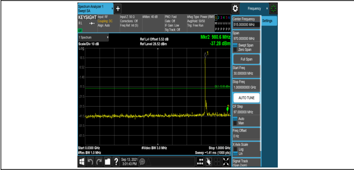
Band26-10MHz-QPSK-26915-1RB#0-Range3:30~1000MHz
