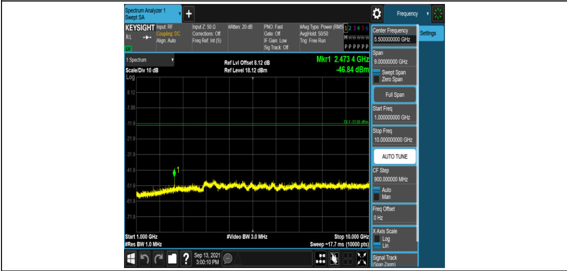
Band26-10MHz-QPSK-26840-1RB#0-Range4:1000~10000MHz
