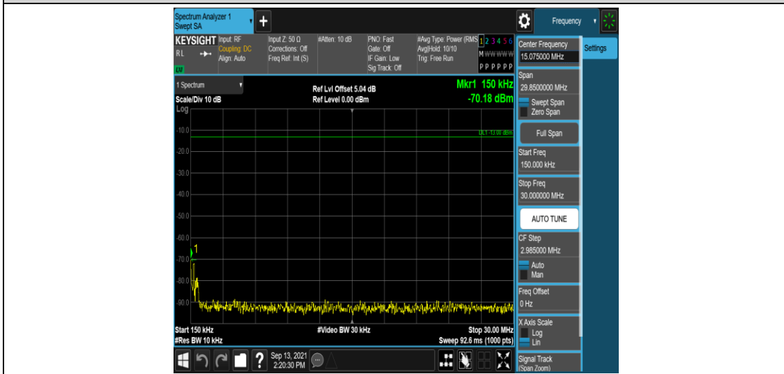
Band26-3MHz-16QAM-27025-1RB#0-Range2:0.15~30MHz
