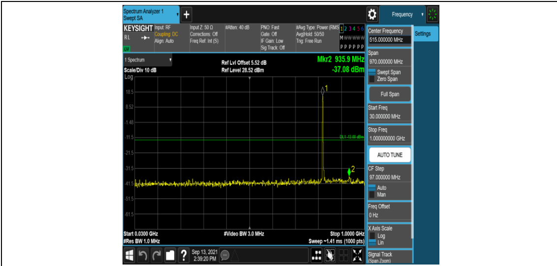
Band26-5MHz-16QAM-26815-1RB#0-Range3:30~1000MHz
