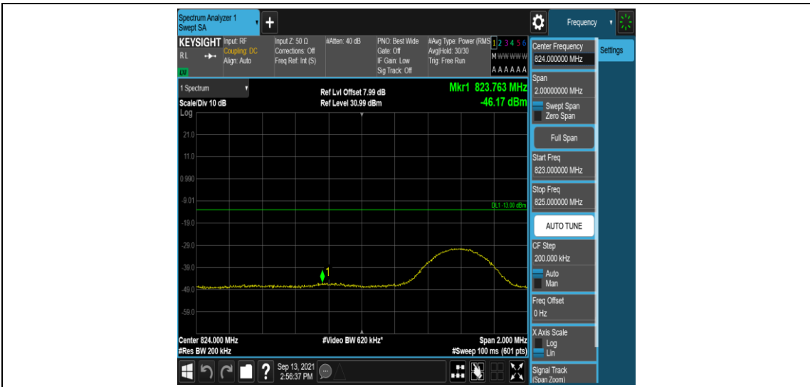
Band26-10MHz-QPSK-26840-1RB#49
