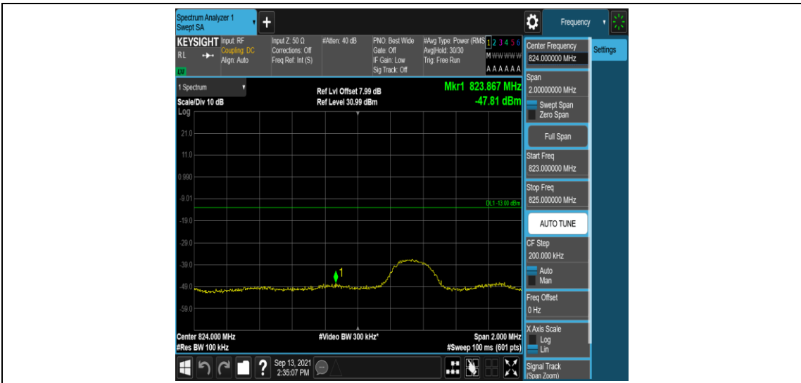
Band26-5MHz-QPSK-26815-1RB#24
