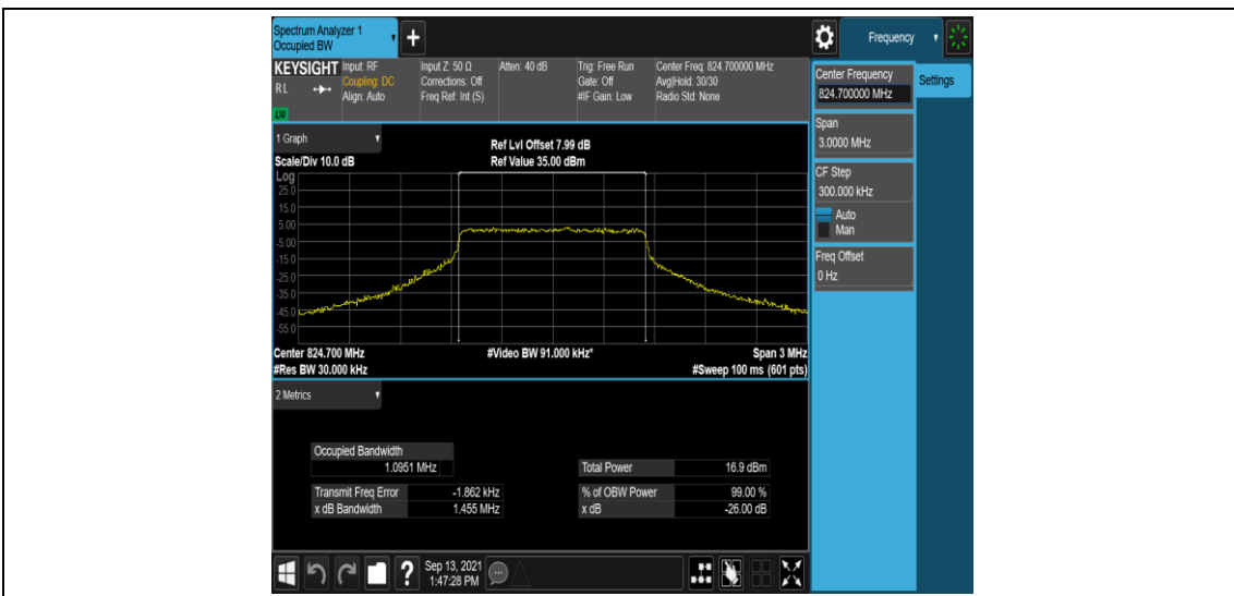
Band26-1.4MHz-QPSK-26797-6RB#0
