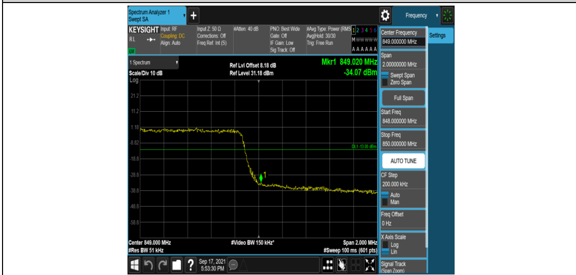
Band26-3MHz-16QAM-27025-15RB#0
