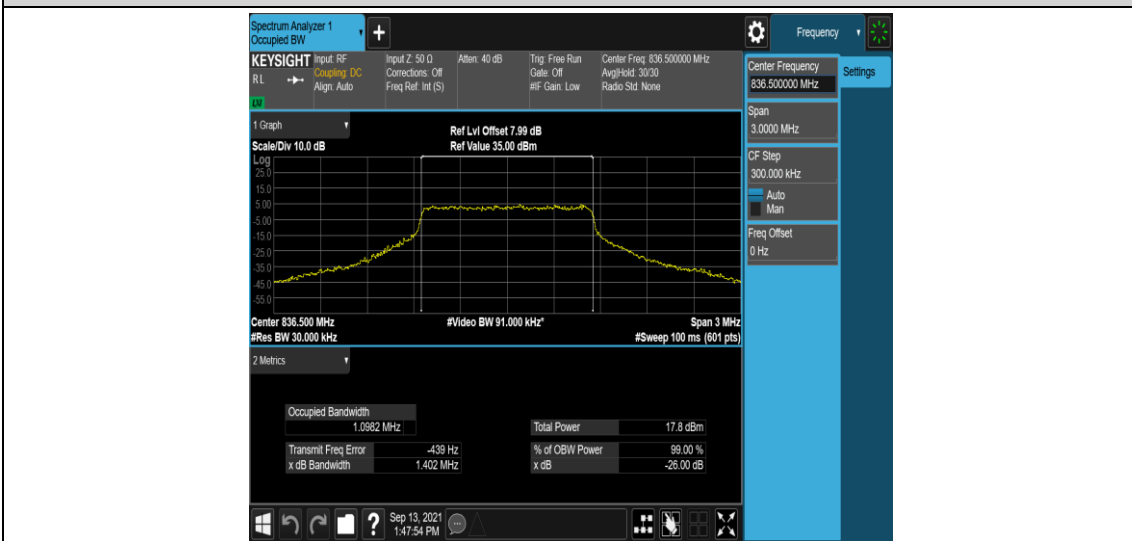
Band26-1.4MHz-QPSK-26915-6RB#0
