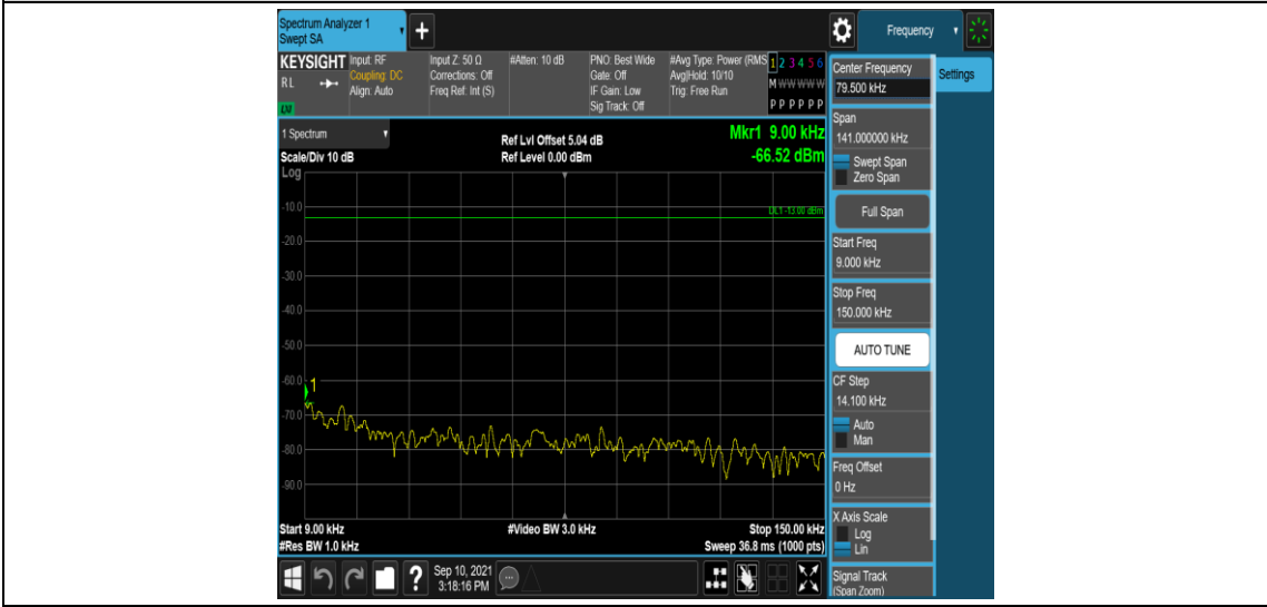
Band26-3MHz-16QAM-26740-1RB#0-Range1:0.009~0.15MHz
