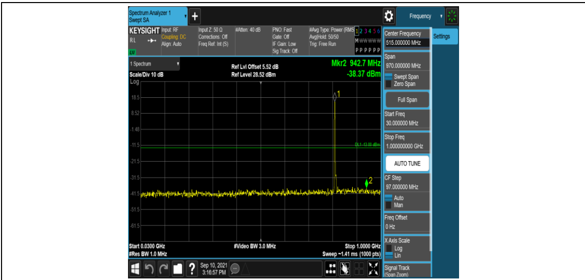
Band26-3MHz-16QAM-26705-1RB#0-Range3:30~1000MHz
