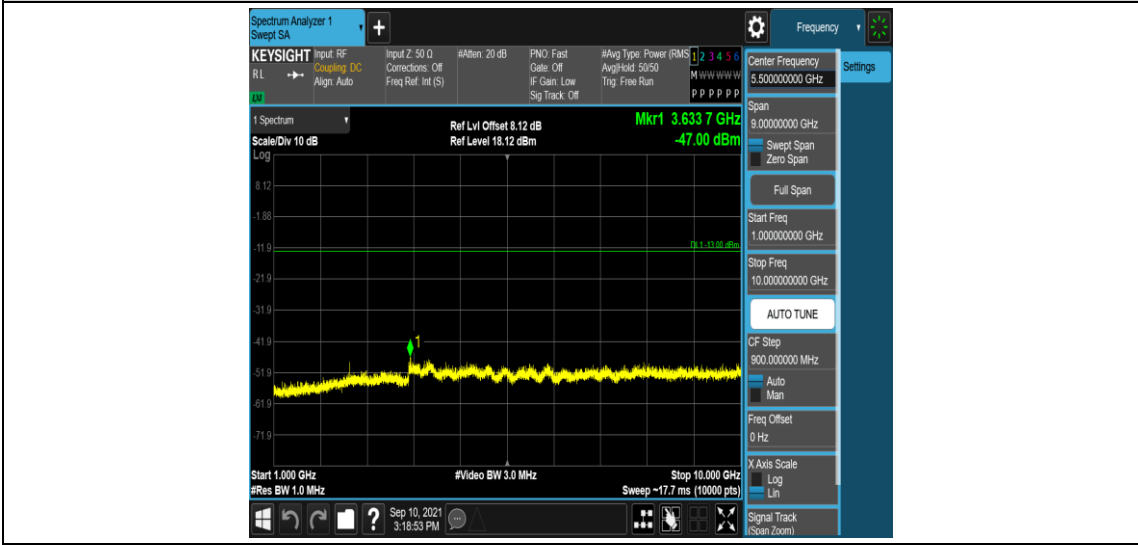
Band26-3MHz-16QAM-26740-1RB#0-Range4:1000~10000MHz
