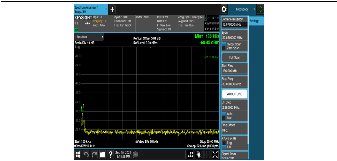
Band26-3MHz-16QAM-26740-1RB#0-Range2:0.15~30MHz
