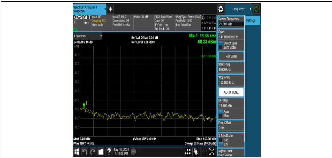
Band26-3MHz-QPSK-26775-1RB#0-Range1:0.009~0.15MHz
