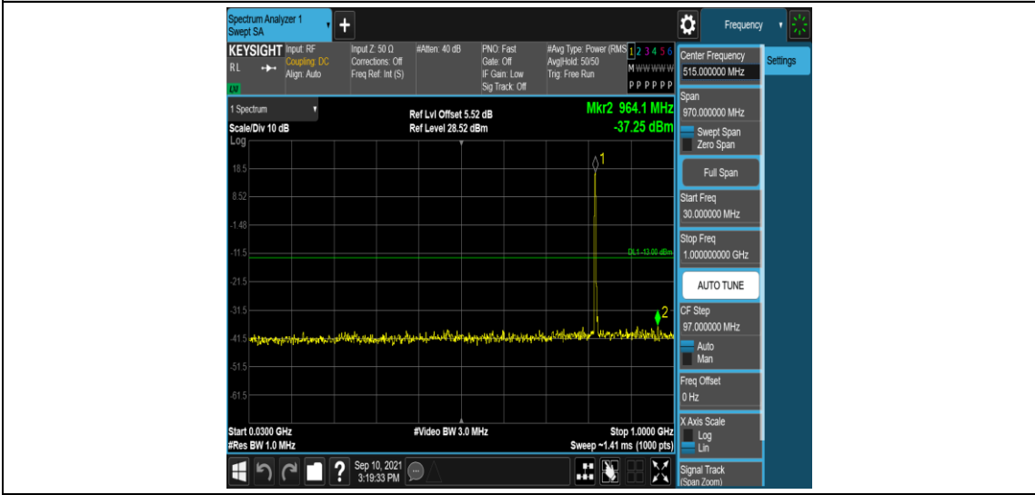
Band26-3MHz-QPSK-26775-1RB#0-Range3:30~1000MHz
