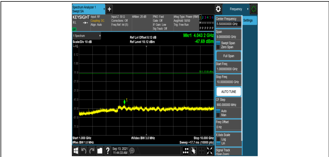
Band26-5MHz-16QAM-26765-1RB#0-Range4:1000~10000MHz
