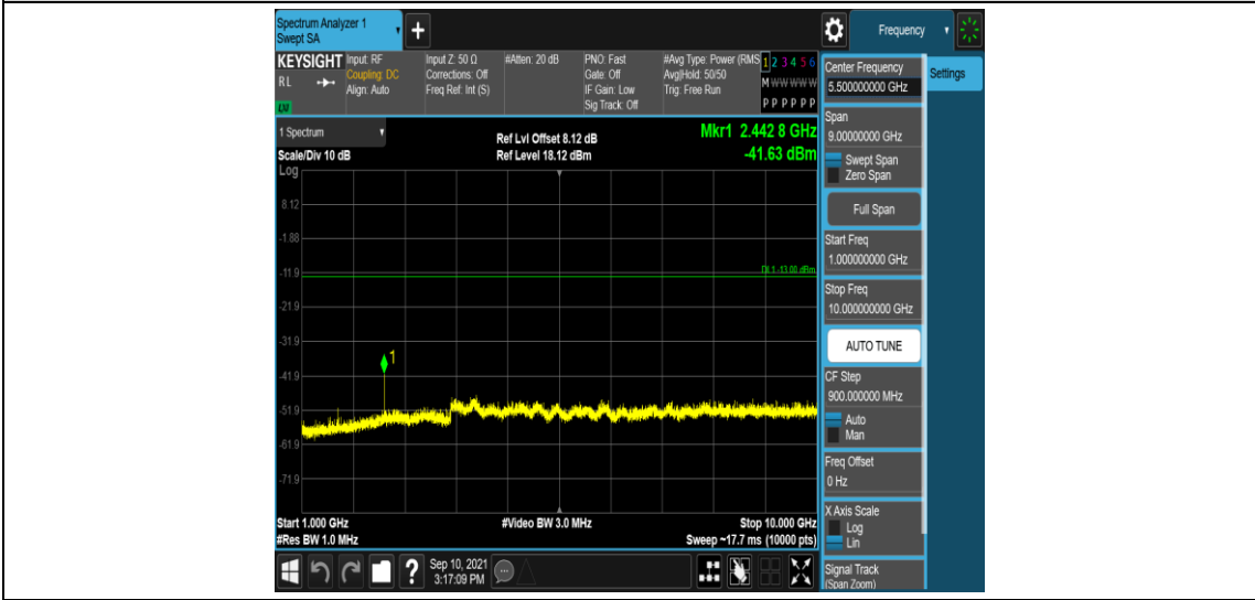
Band26-3MHz-16QAM-26705-1RB#0-Range4:1000~10000MHz
