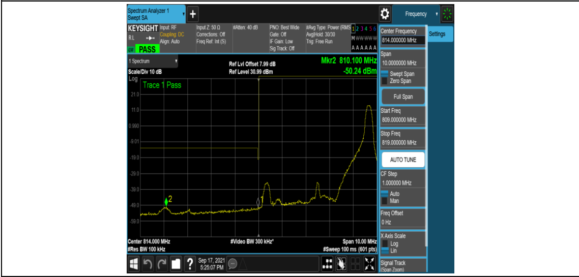
Band26-5MHz-QPSK-26715-1RB#24
