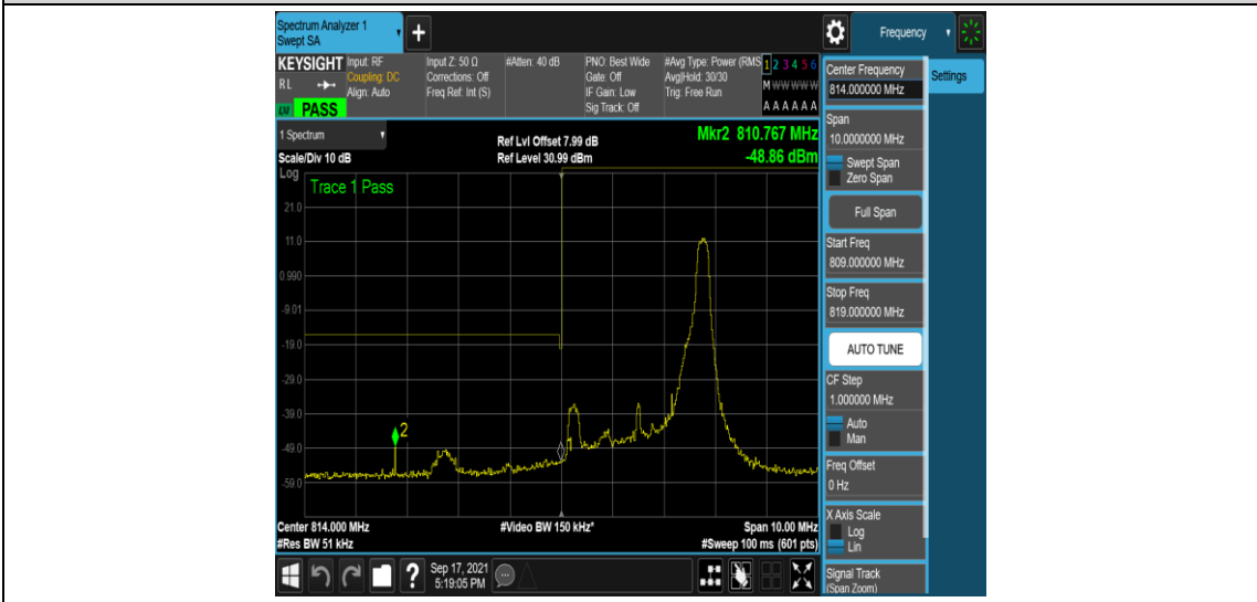
Band26-3MHz-16QAM-26705-1RB#14
