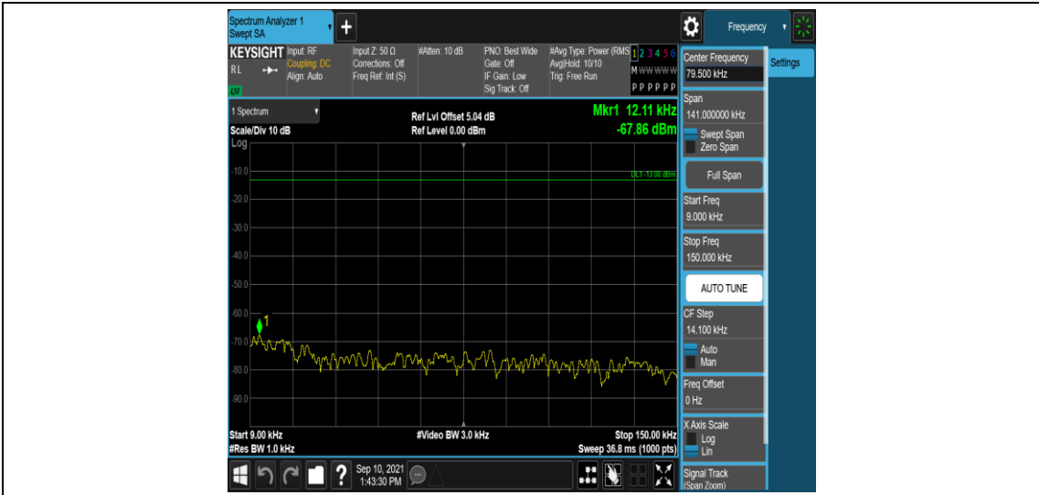
Band26-1.4MHz-QPSK-26783-1RB#0-Range1:0.009~0.15MHz
