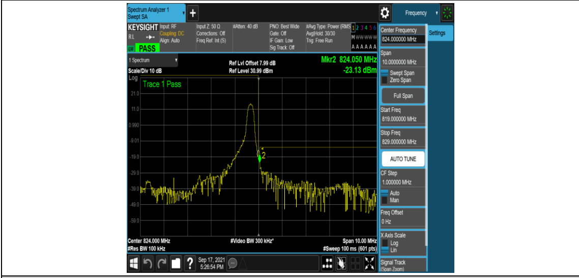
Band26-5MHz-QPSK-26765-1RB#24
