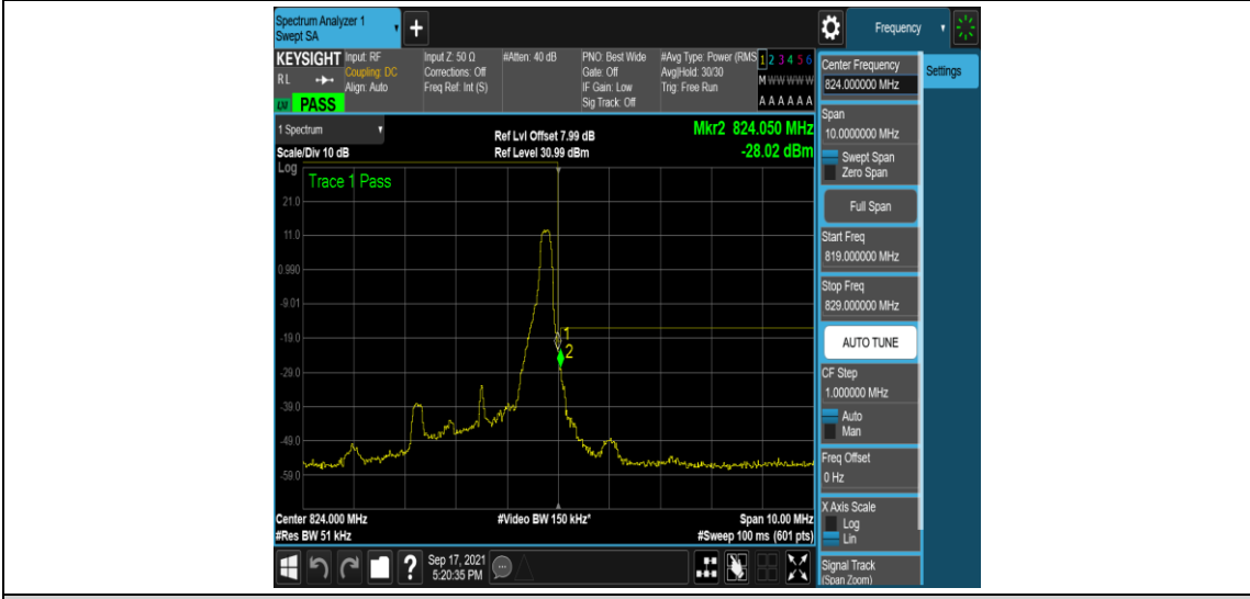
Band26-3MHz-QPSK-26775-1RB#14
